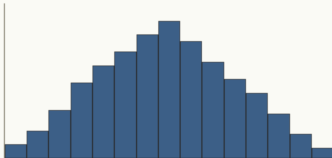
Bell-shaped
