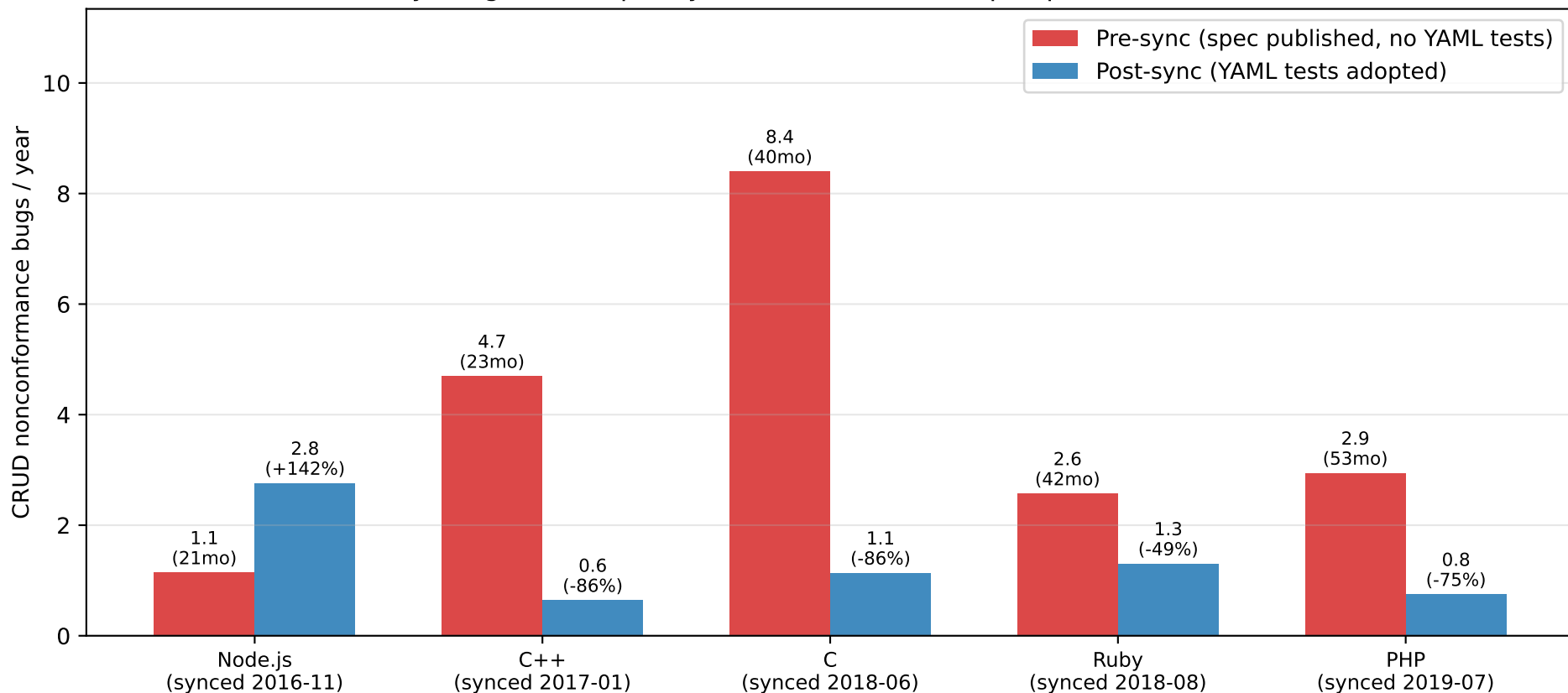
CRUD bug rate/year before vs. after YAML test adoption 5 late-syncing drivers; pre-sync window starts at spec publication (Feb 2015)
