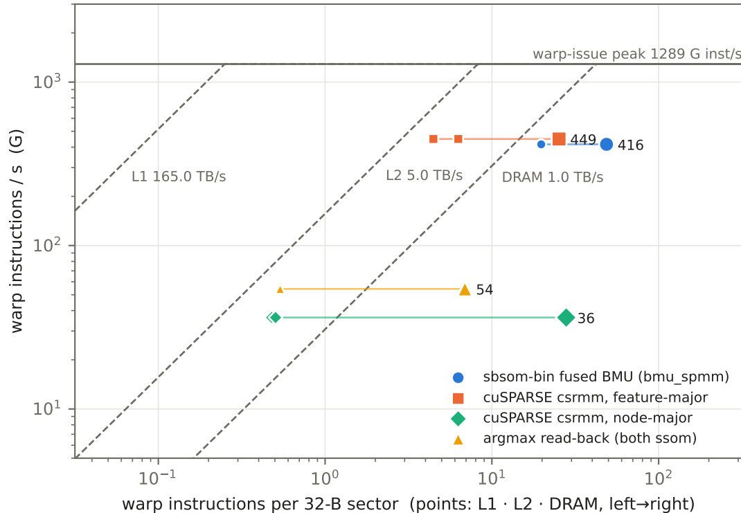
Instruction roofline — BMU phase, 128×128
