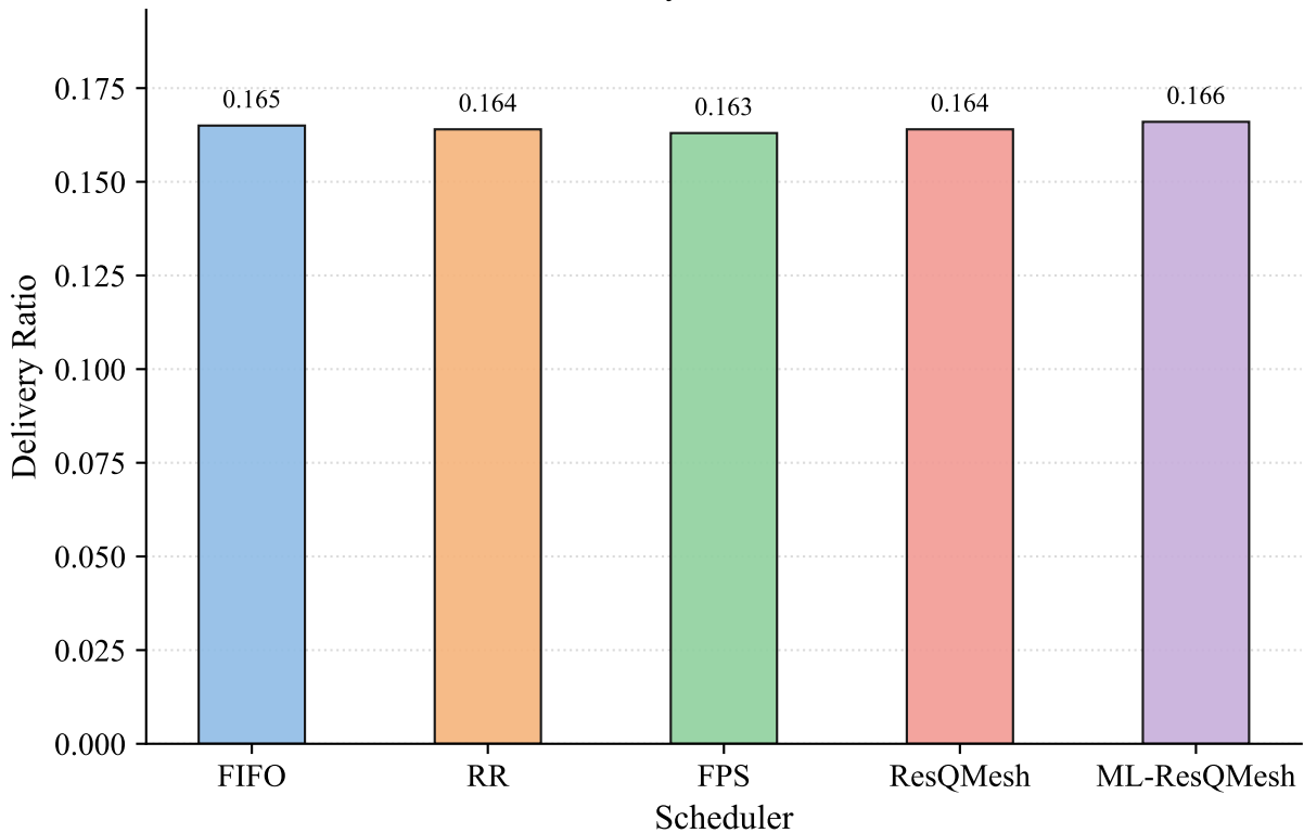
Delivery Ratio - Burst
