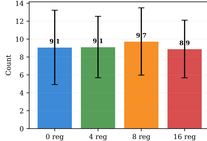
(c) Aligned Attention Heads ( \rho > 0.5 per head)
