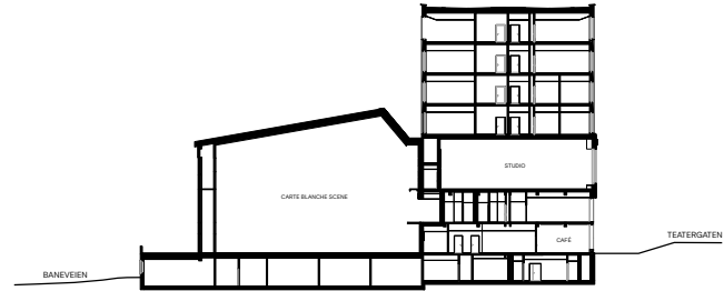
SECTION AA | PROPOSAL
