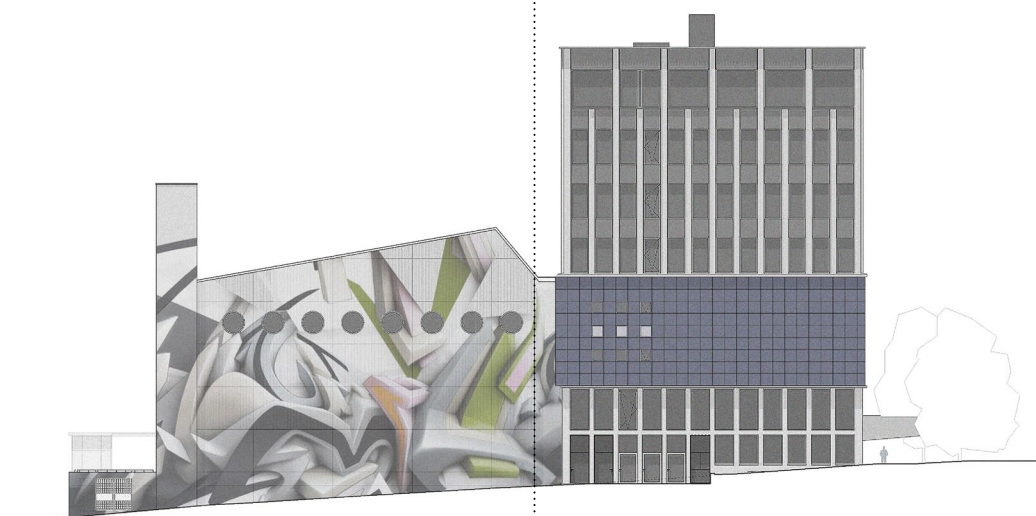
SOUTHWEST ELEVATION HÅKONSGÅTEN STREET
