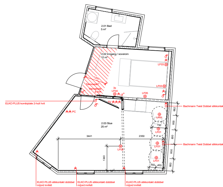
ELECTRICAL INSTALLATION
