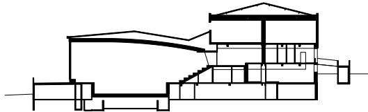
SECTION AA | EXISTING
