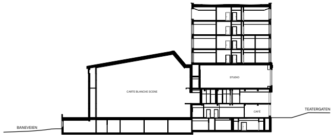
SECTION AA | PROPOSAL
