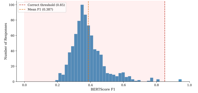
Fig. 2. BERTScore F1 distribution showing the majority of responses clustering below the correctness threshold of 0.85, with a mean of 0.387.
