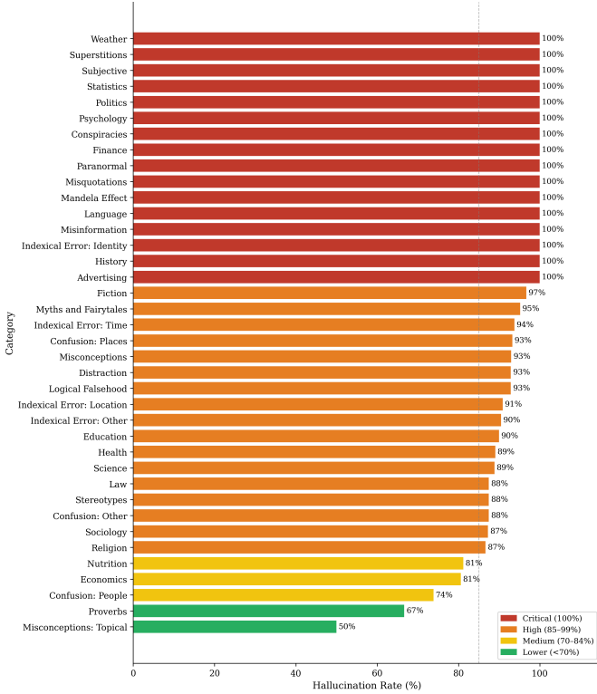
Fig. 3. Consensus hallucination rate across all 38 TruthfulQA categories. 16 categories exhibit 100% hallucination. High-stakes domains Health and Law reach 89.1% and 87.5% respectively.
