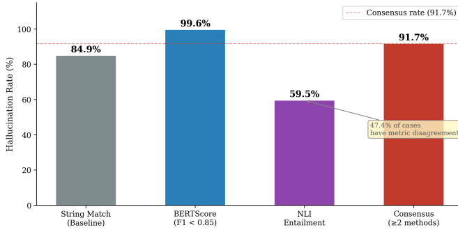
Fig. 1. Hallucination rates across three detection methods and the consensus scheme. The 40.1pp spread demonstrates that metric choice substantially affects reported results.
