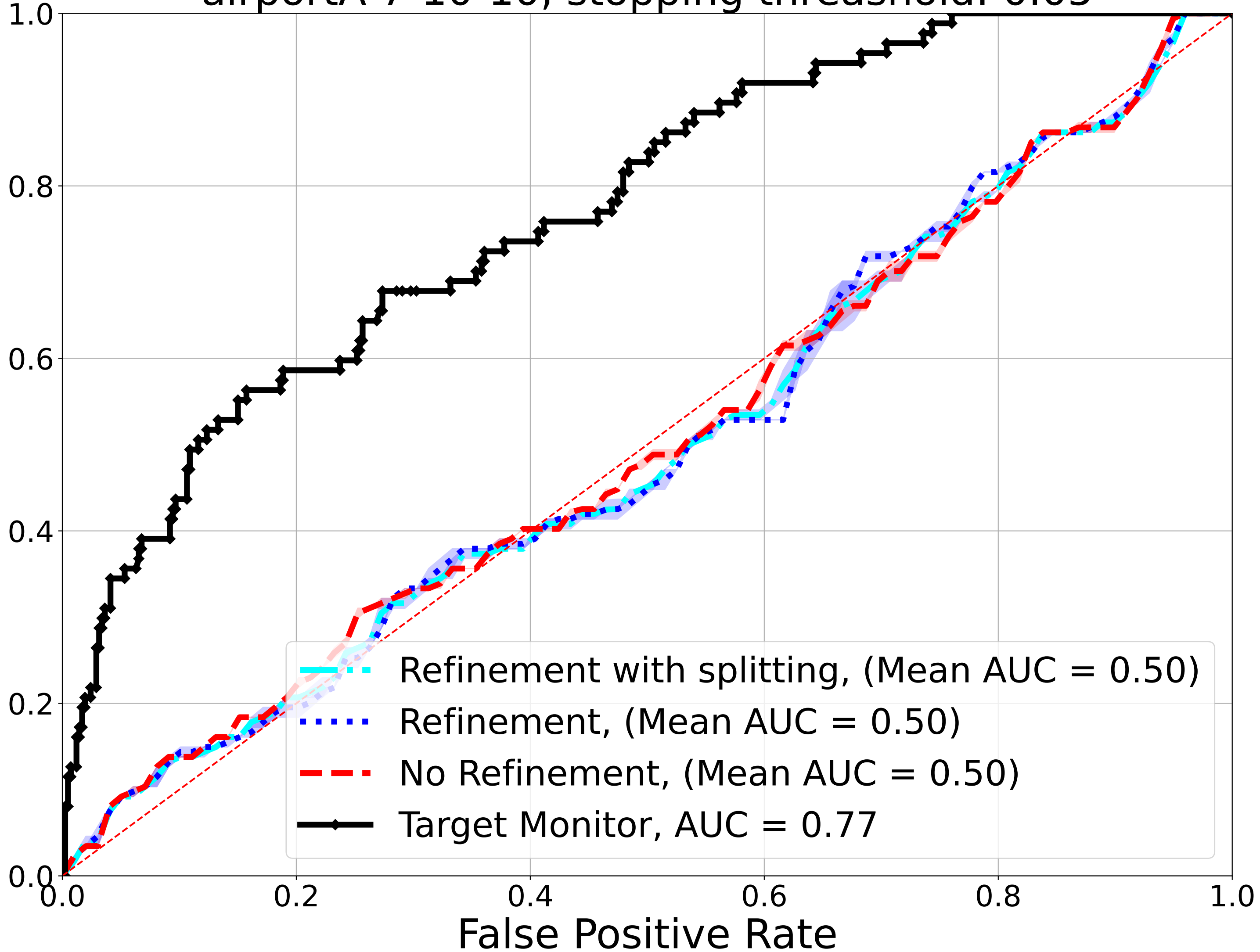
airportA-7-10-10, stopping threshold: 0.05
