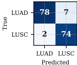
Gated ABMIL (GigaPath)
