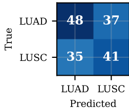
RBF-SVM
