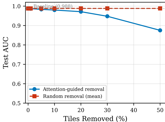
AUC vs. Tile Removal
