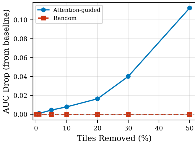
AUC Drop vs. Tile Removal
