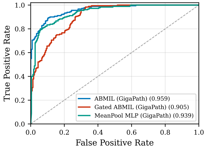
ROC Curves — CPTAC (External Validation)
