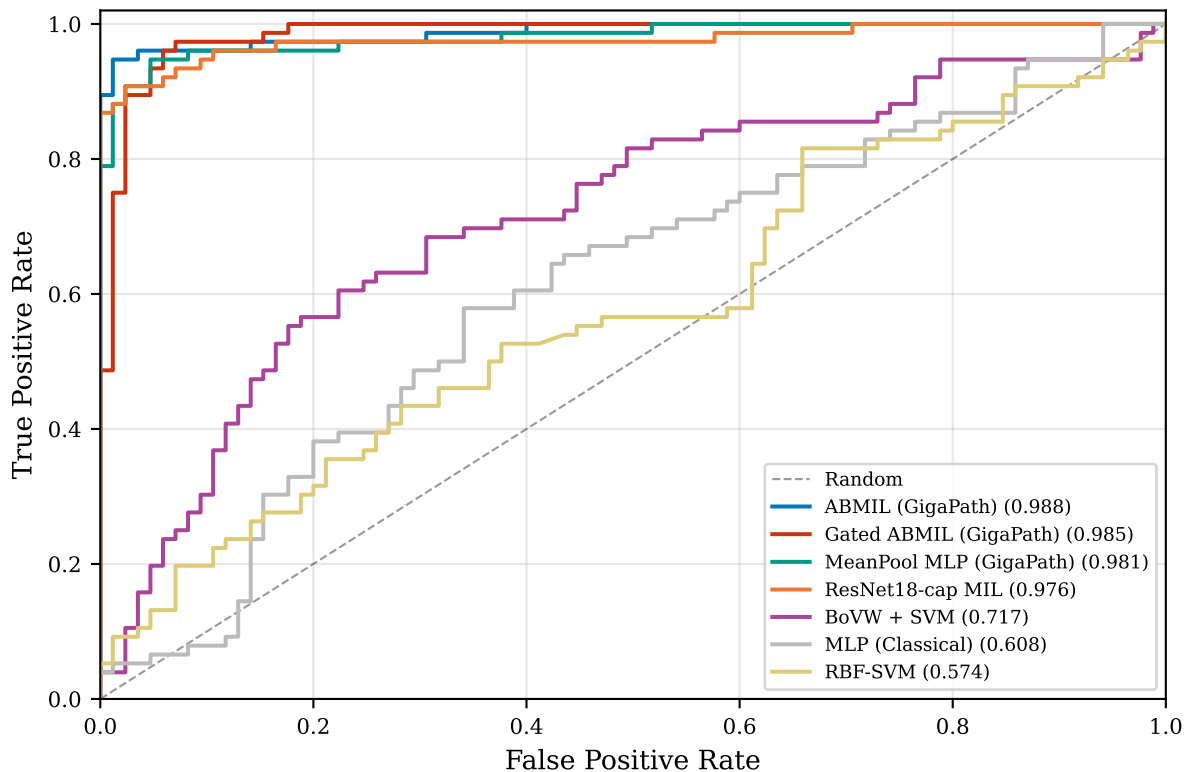
ROC Curves — Test Set
