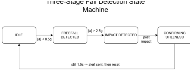
Fig. 2. Three-stage fall-detection finite-state machine.
