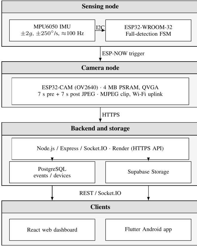
Fig. 1. C.A.S.C.O. system architecture.
