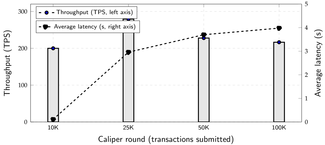
Figure 4.6: Blockchain throughput (bars, left axis) and average latency (dashed line, right axis) across the four Hyperledger Caliper benchmark rounds. Throughput remains in the 200–280 TPS band across all rounds, while average latency degrades non-linearly as the round size approaches the Fabric Gateway’s default concurrency limit (500 connections). Data values are taken directly from Table 4.7.
