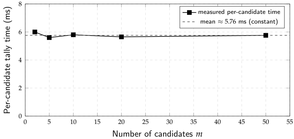
Figure 4.4: Per-candidate tally time as the number of candidates m varies from 2 to 50, with the voter count fixed at n = 1,000 . The measured points fluctuate only within \pm 0.4 ms around the mean (5.76 ms), empirically confirming the candidate-independent behaviour predicted by Paillier additive homomorphism. Data taken from Table 4.5.
