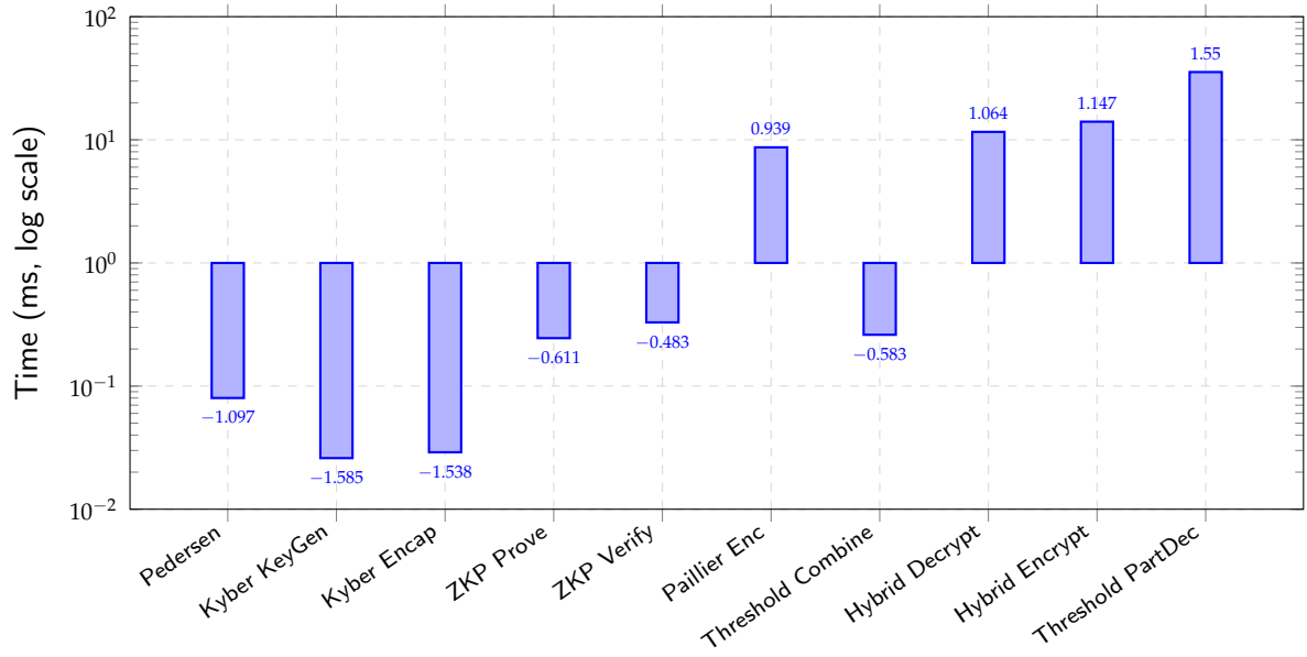
Figure 4.1: Per-operation cost of every cryptographic primitive in the proposed framework, plotted on a logarithmic time axis. Values are taken directly from Table 4.2; the three-orders-of-magnitude span justifies the log-scale presentation.
