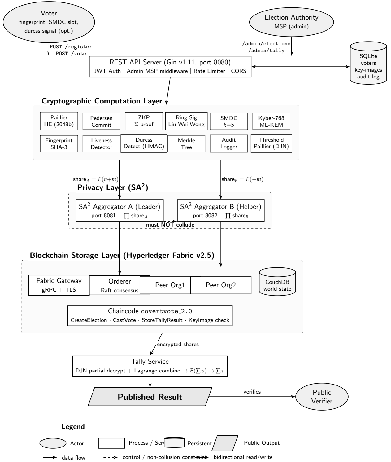
Figure 3.1: End-to-end system architecture of the proposed framework. The diagram traces the full path from voter authentication through the cryptographic pipeline, the two non-colluding SA 2 aggregators, the Hyperledger Fabric storage layer, and the threshold tally service to the published result. All shapes and line styles are distinguishable in greyscale.
