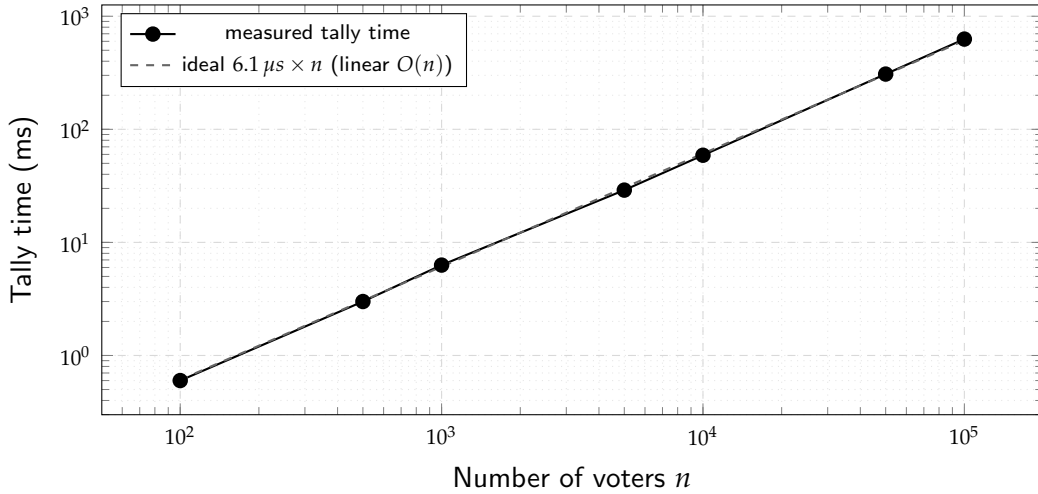
Figure 4.3: Homomorphic tally time versus voter count, plotted on a log-log scale. The measured points lie almost exactly on the dashed reference line 6.1 \mu\text{s} \times n , empirically confirming O(n) complexity with a constant per-vote cost across four orders of magnitude (100 to 100,000 voters). Data values are taken directly from Table 4.4.
