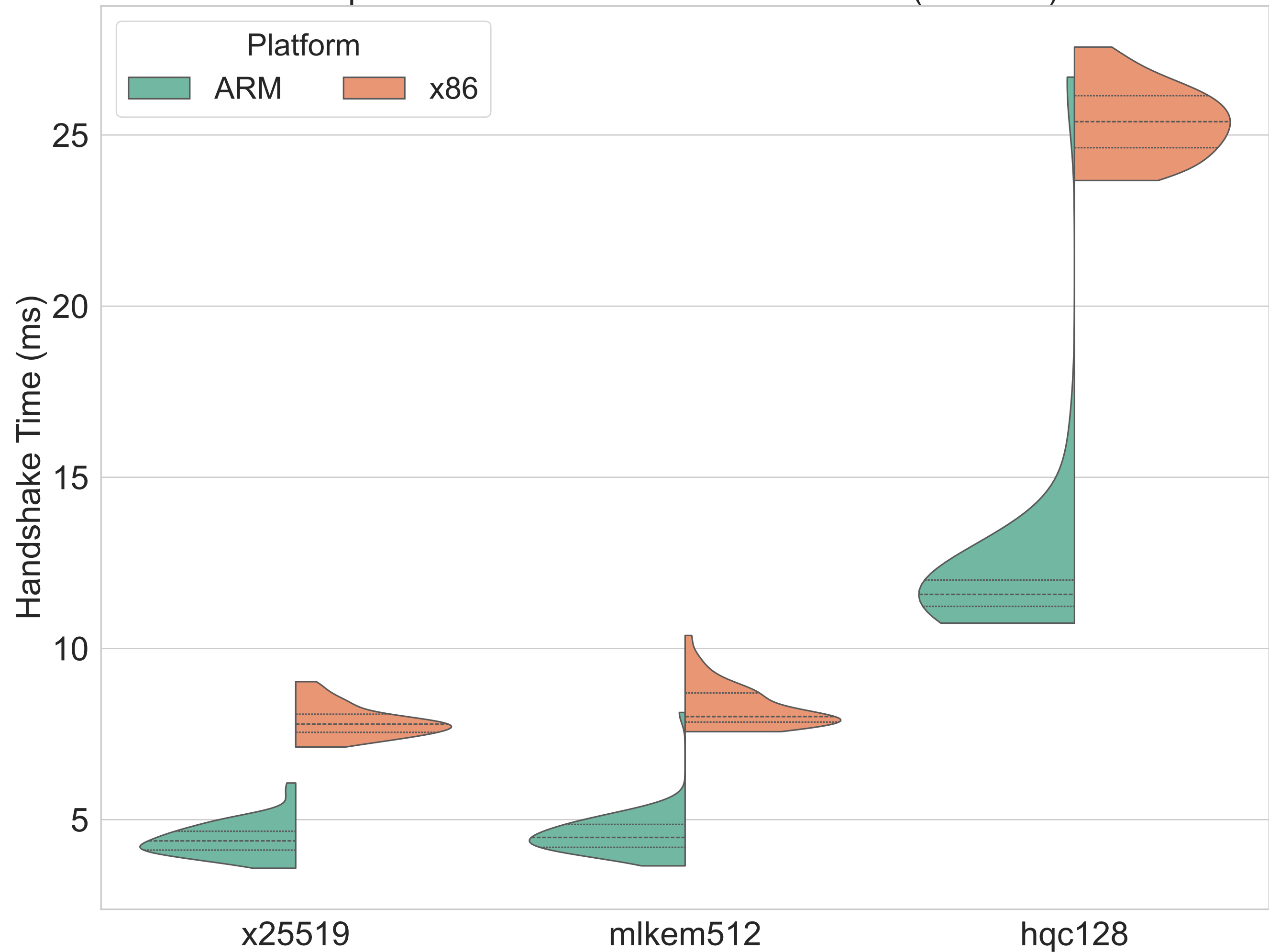
Impact of KEM on TLS Handshake Time (mldsa44)
