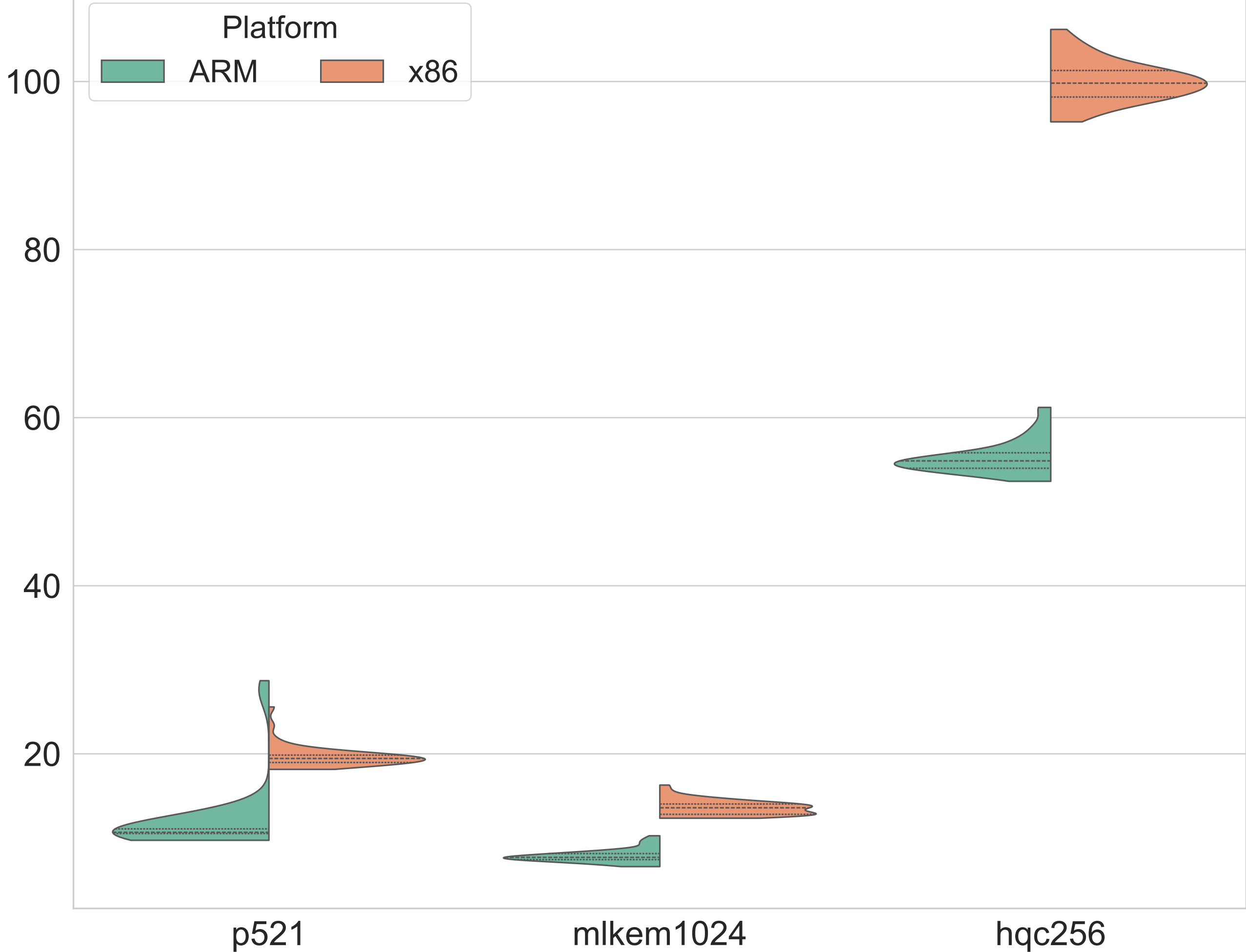
Impact of KEM on TLS Handshake Time (mldsa87)
