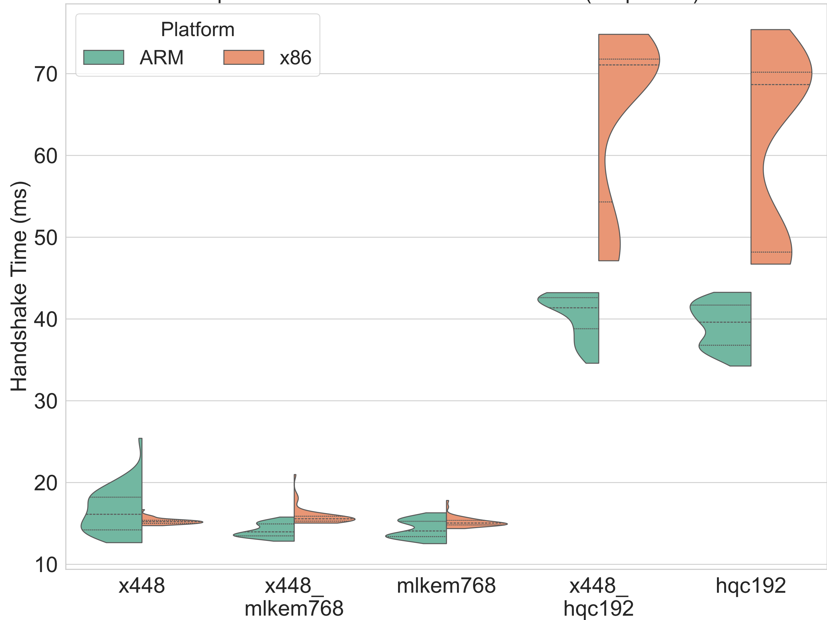
Impact of KEM on TLS Handshake Time (secp384r1)
