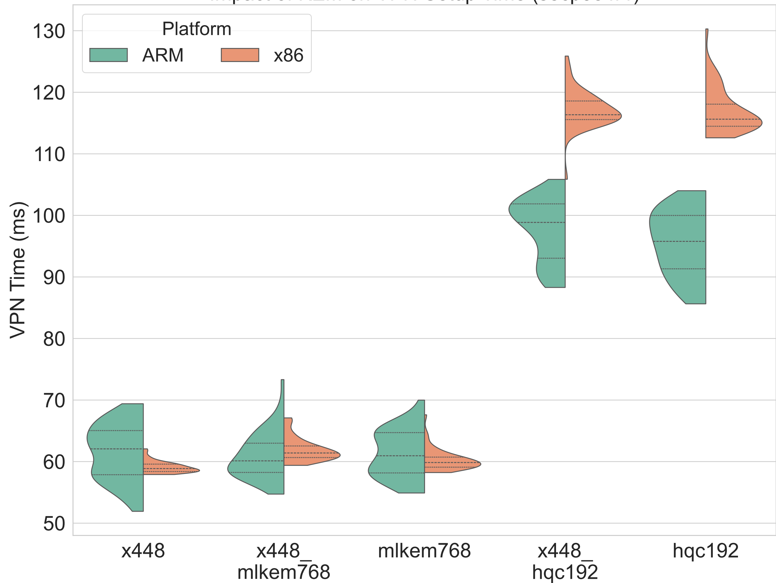
Impact of KEM on VPN Setup Time (secp384r1)
