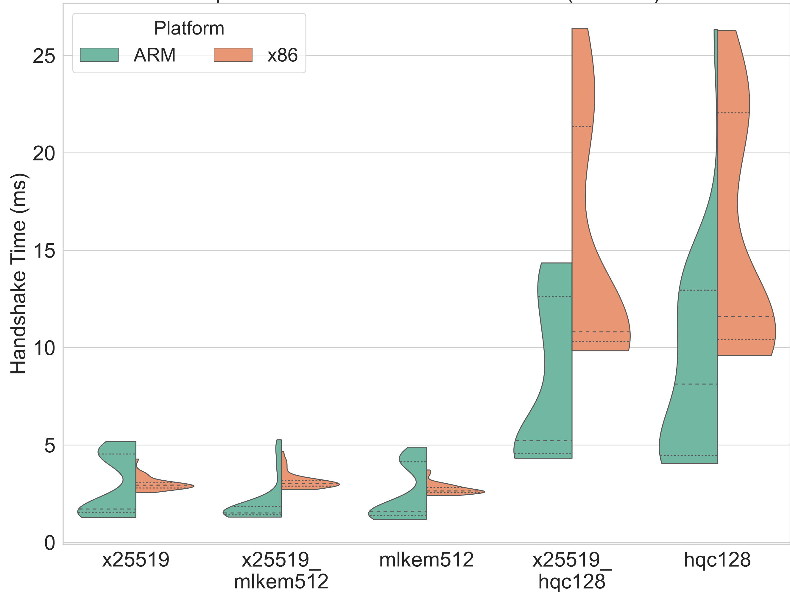
Impact of KEM on TLS Handshake Time (ed25519)
