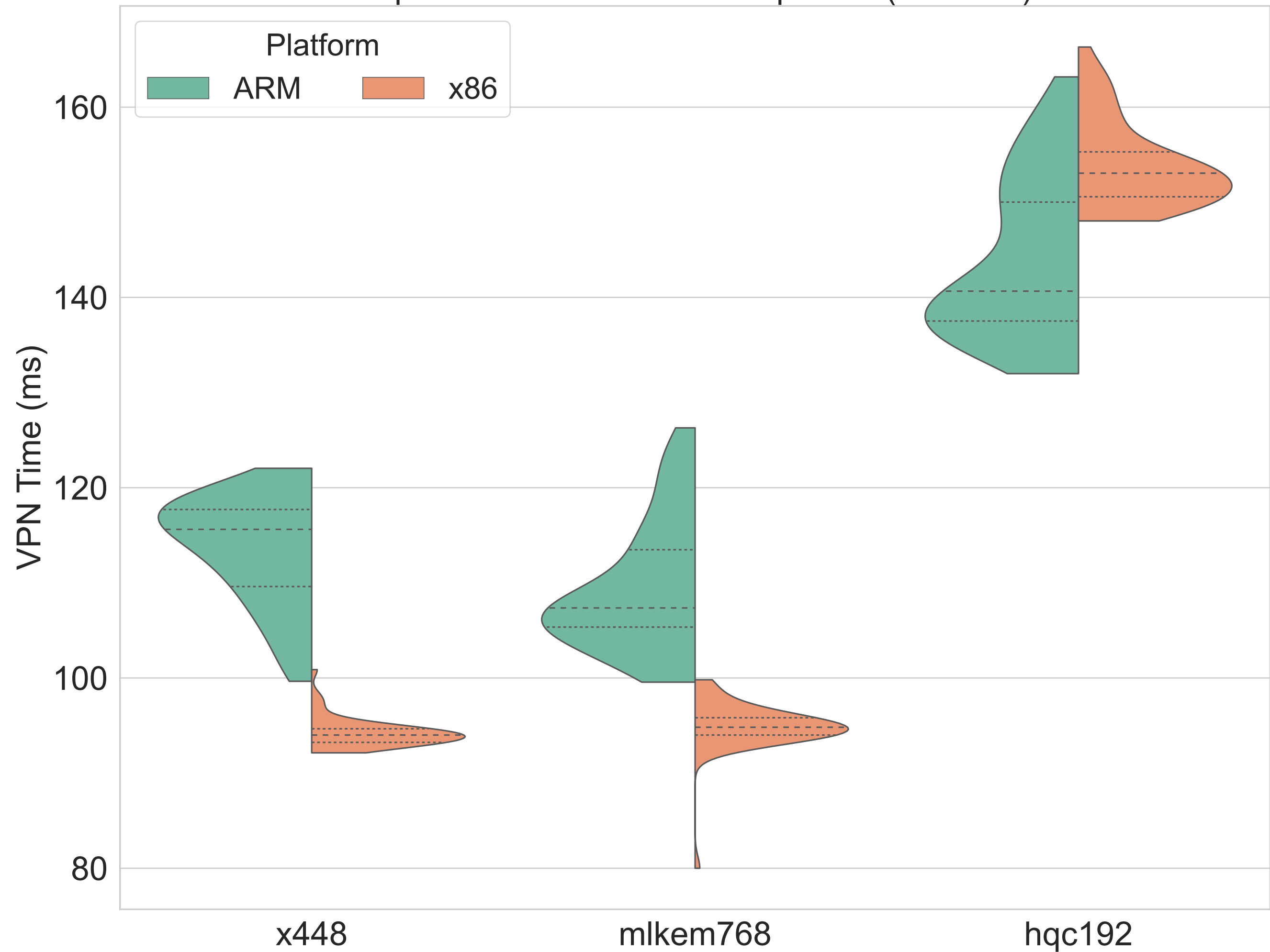
Impact of KEM on VPN Setup Time (mldsa65)
