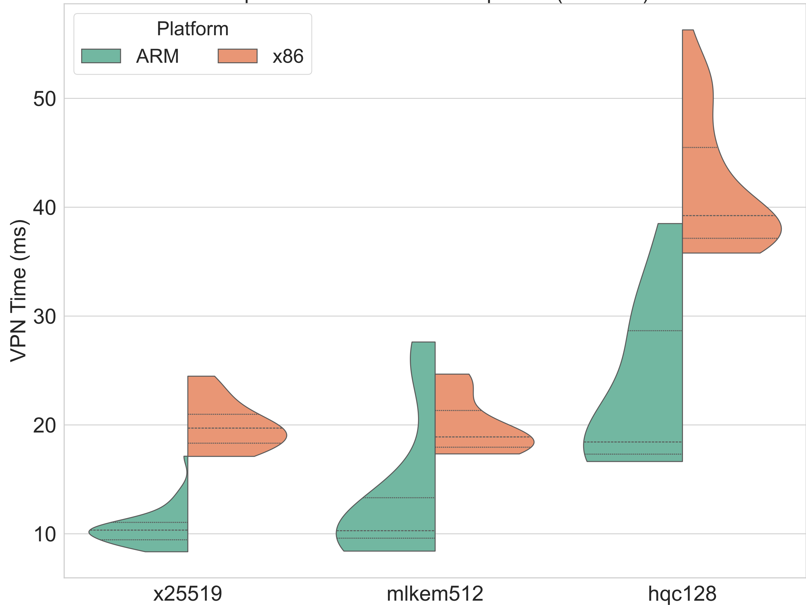
Impact of KEM on VPN Setup Time (mlds44)
