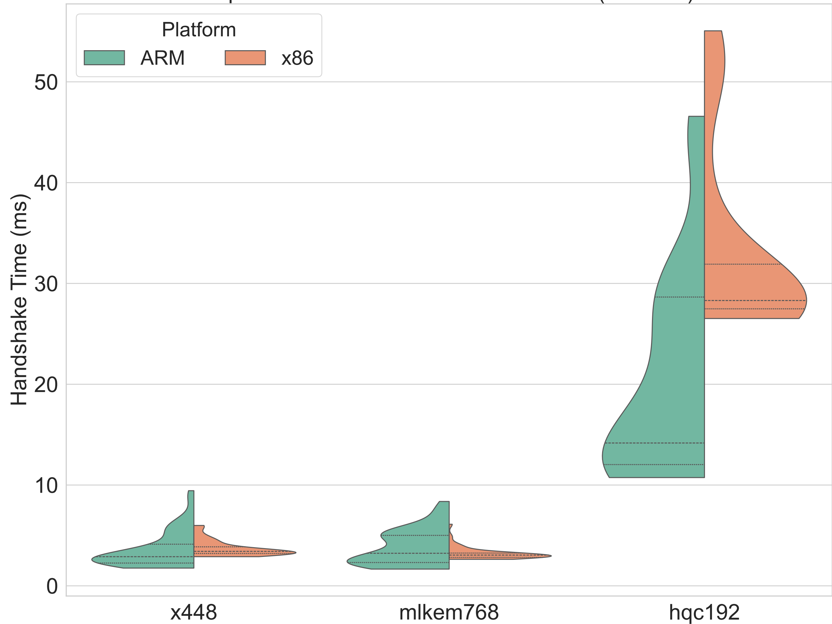
Impact of KEM on TLS Handshake Time (mlds65)
