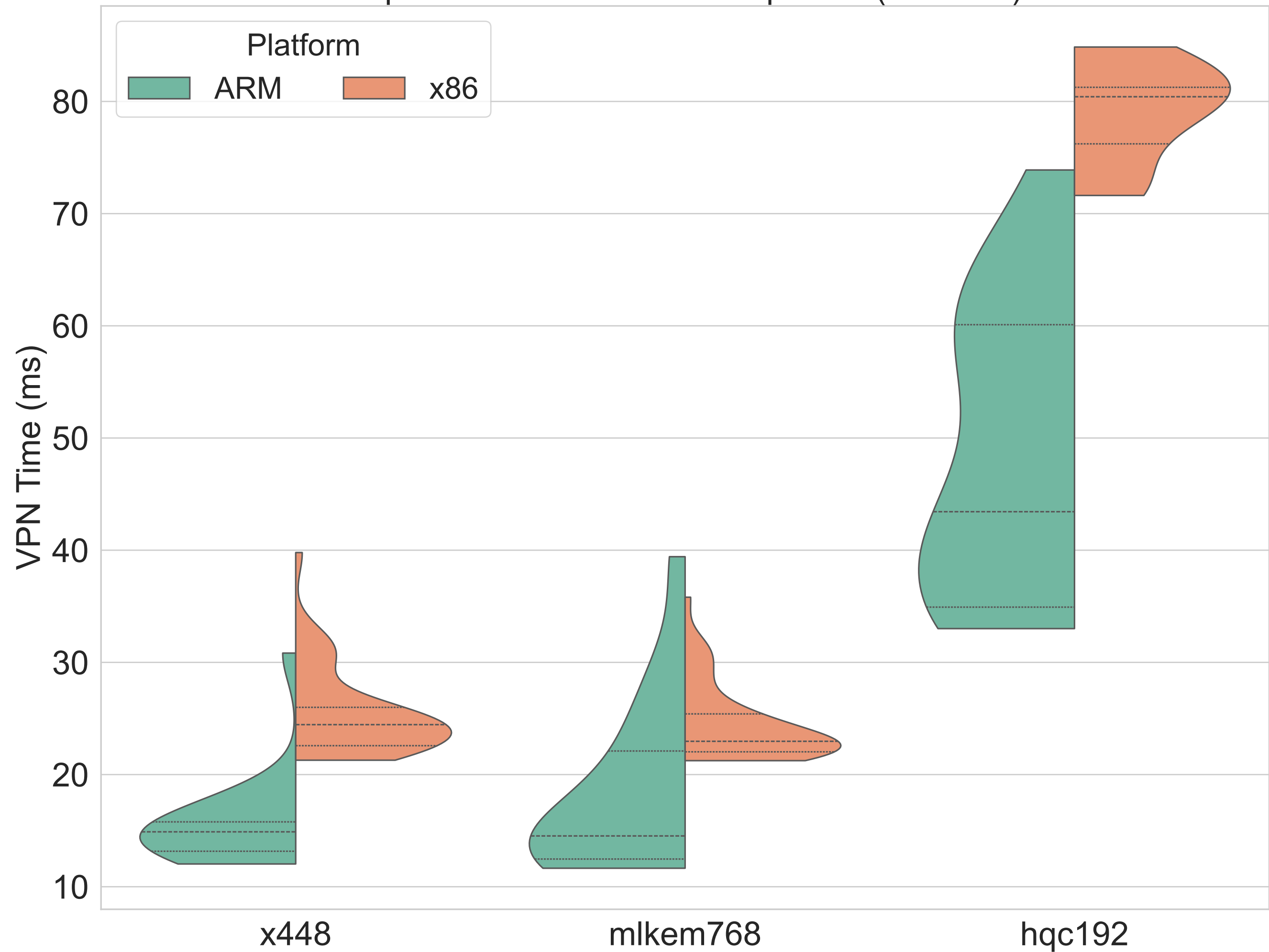
Impact of KEM on VPN Setup Time (mlds65)
