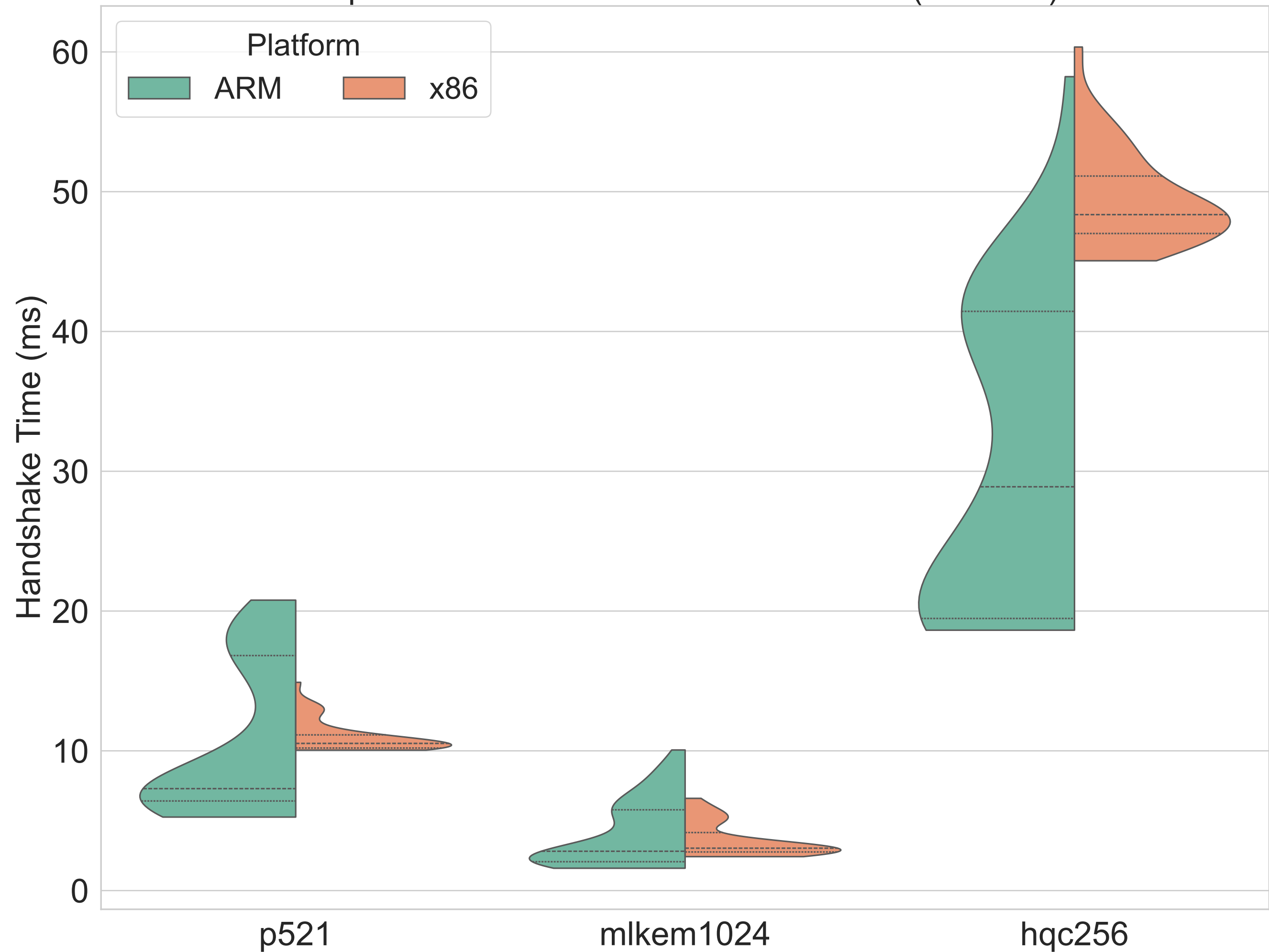
Impact of KEM on TLS Handshake Time (mlds87)
