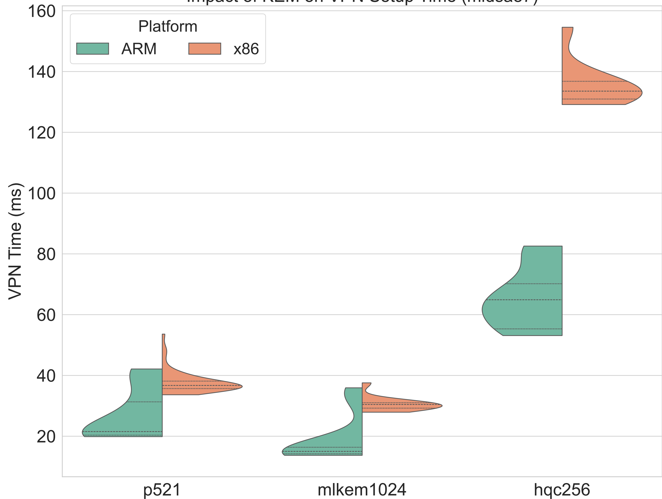
Impact of KEM on VPN Setup Time (mlds87)
