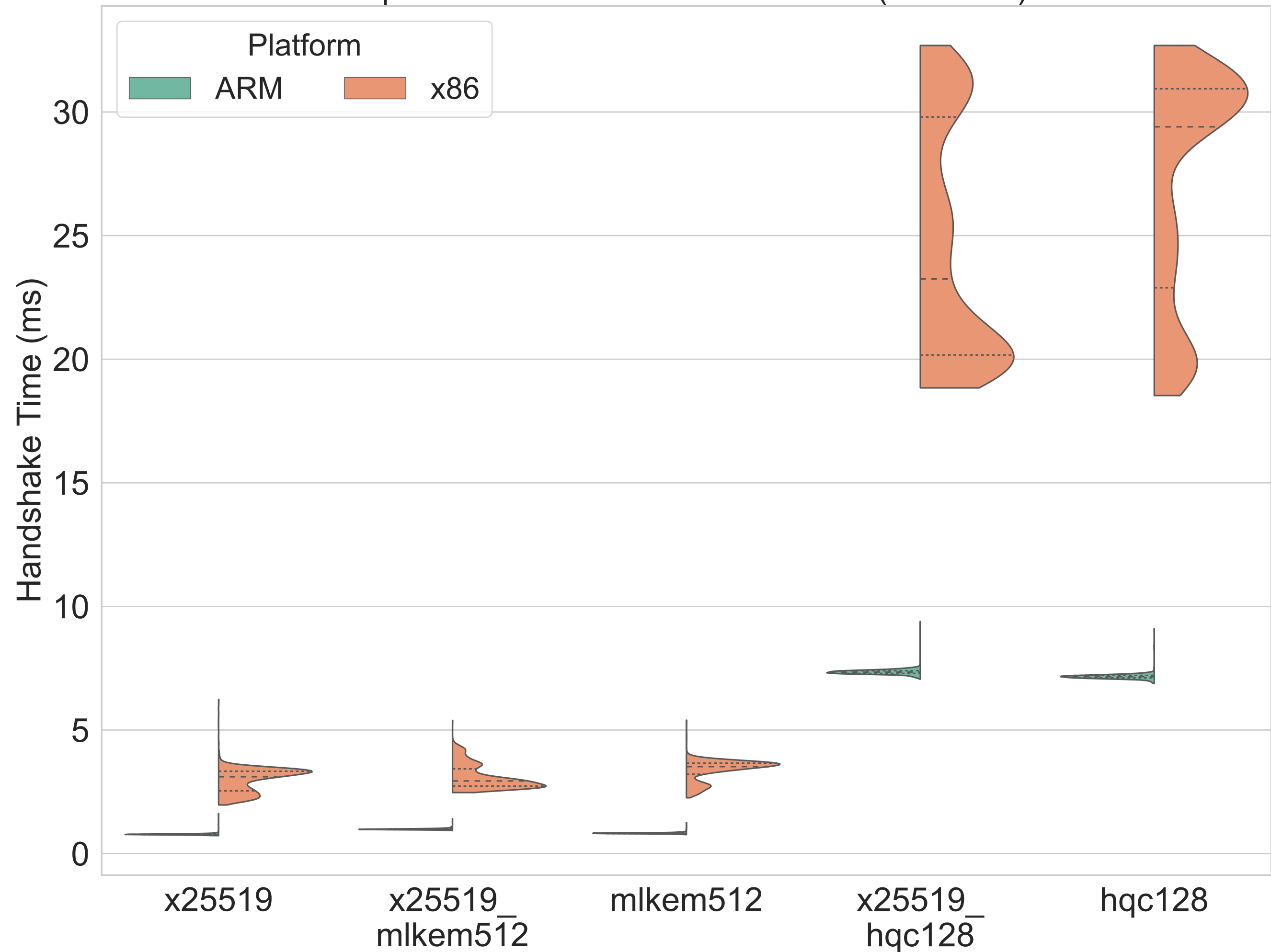
Impact of KEM on Handshake Time (ed25519)
