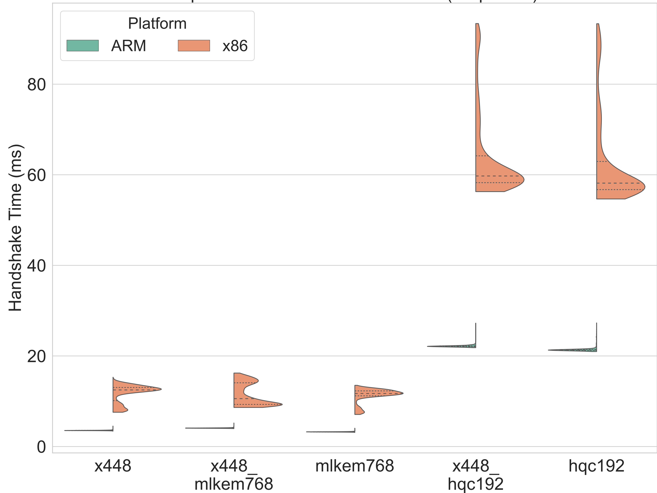
Impact of KEM on Handshake Time (secp384r1)
