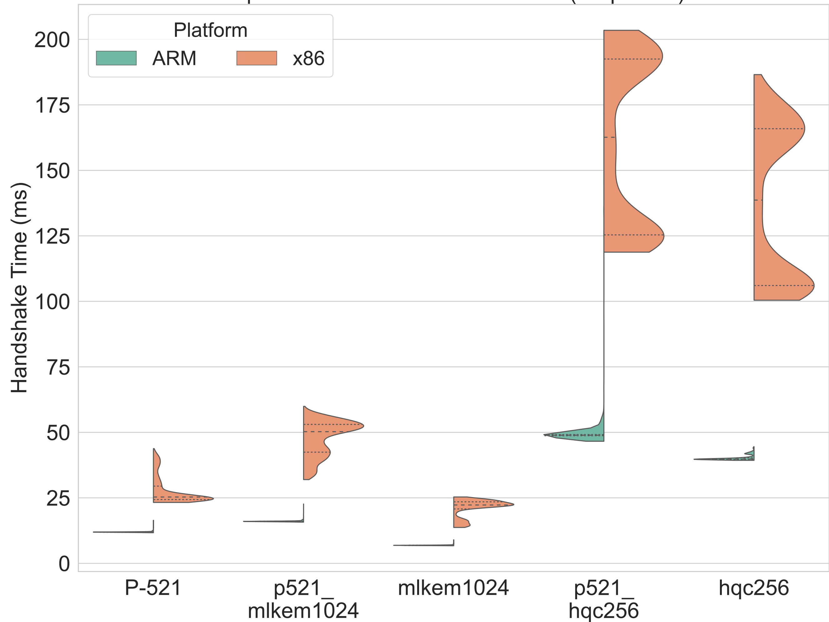
Impact of KEM on Handshake Time (secp521r1)
