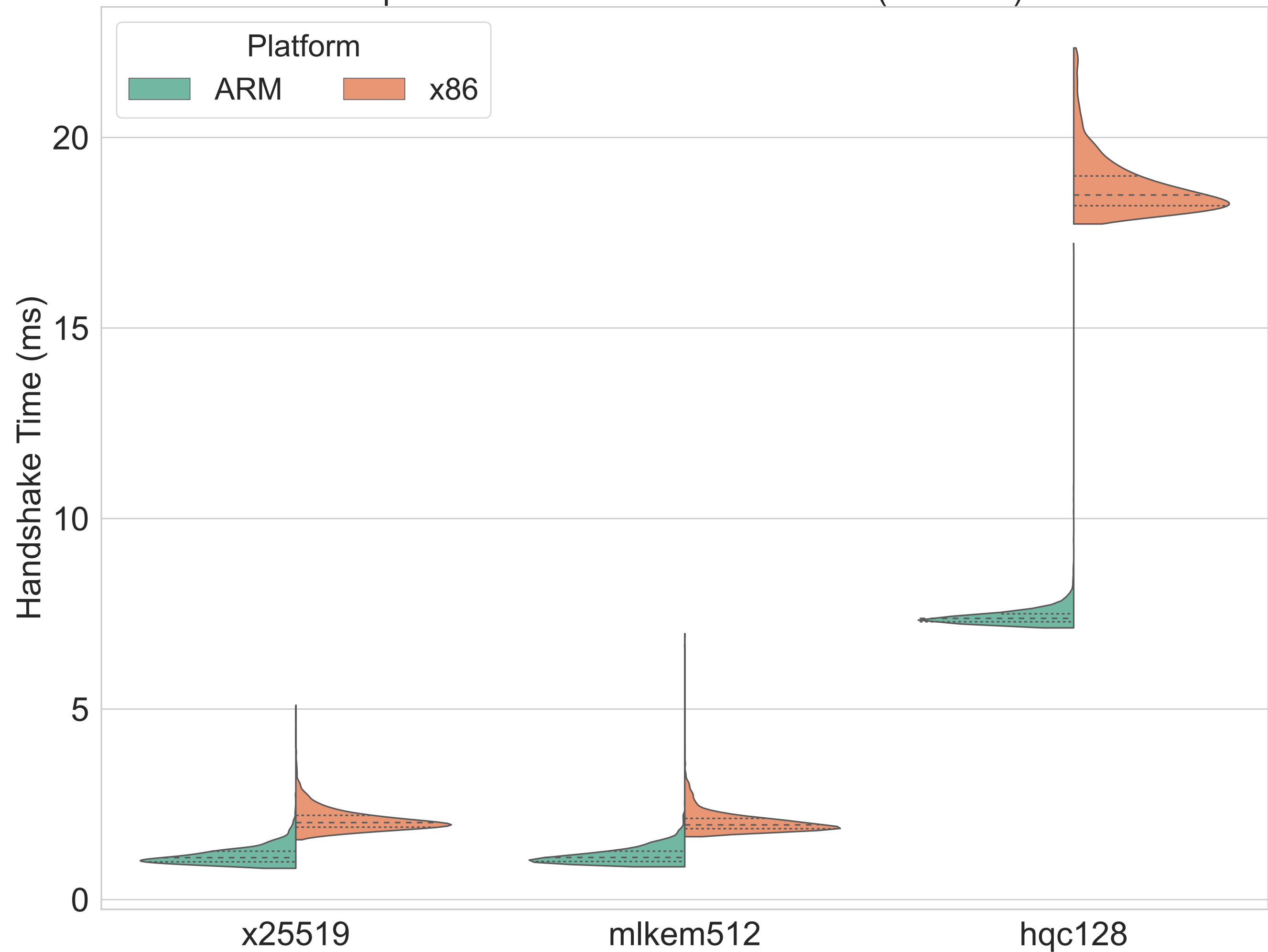
Impact of KEM on Handshake Time (mlds44)
