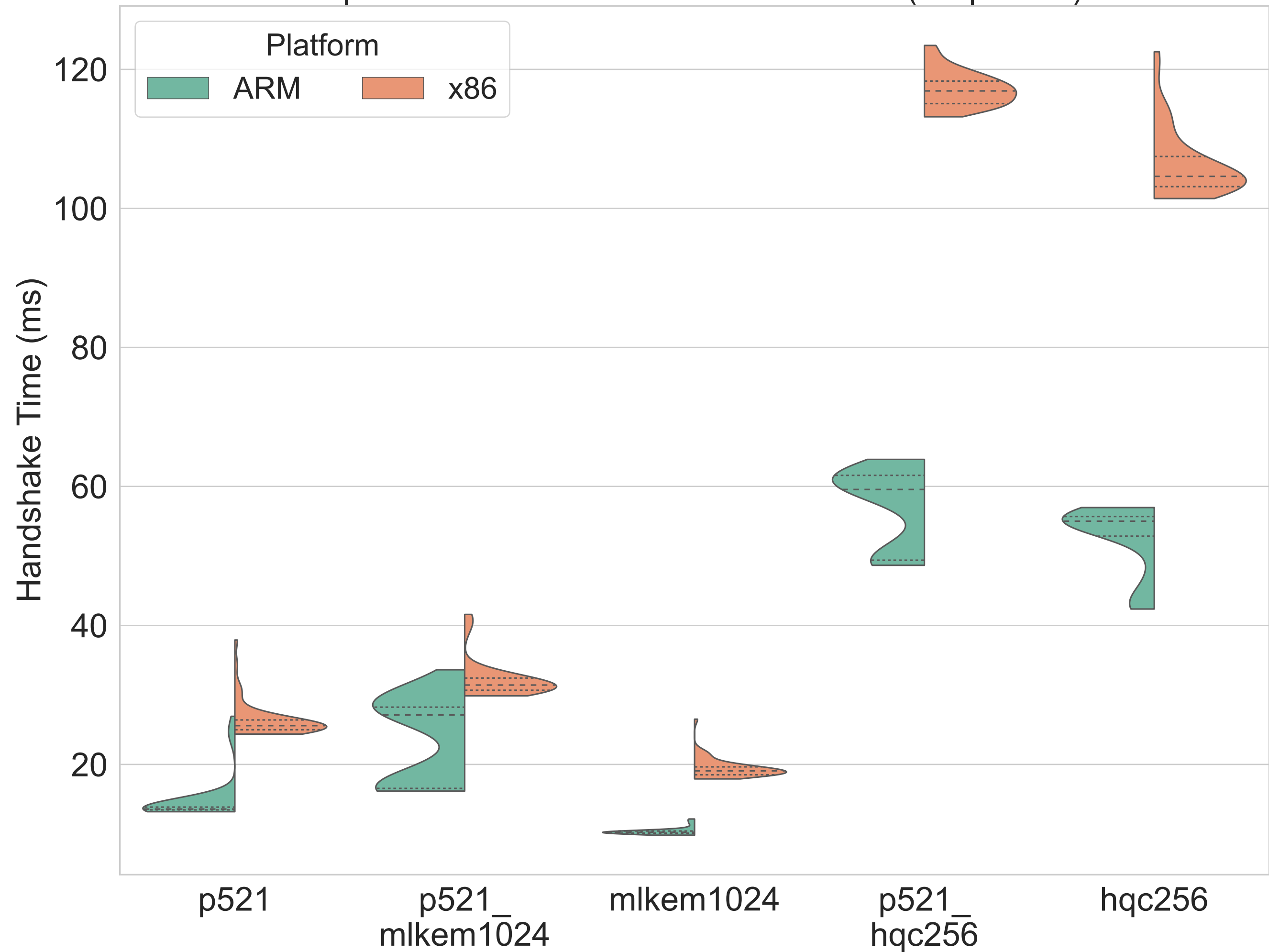
Impact of KEM on TLS Handshake Time (secp521r1)
