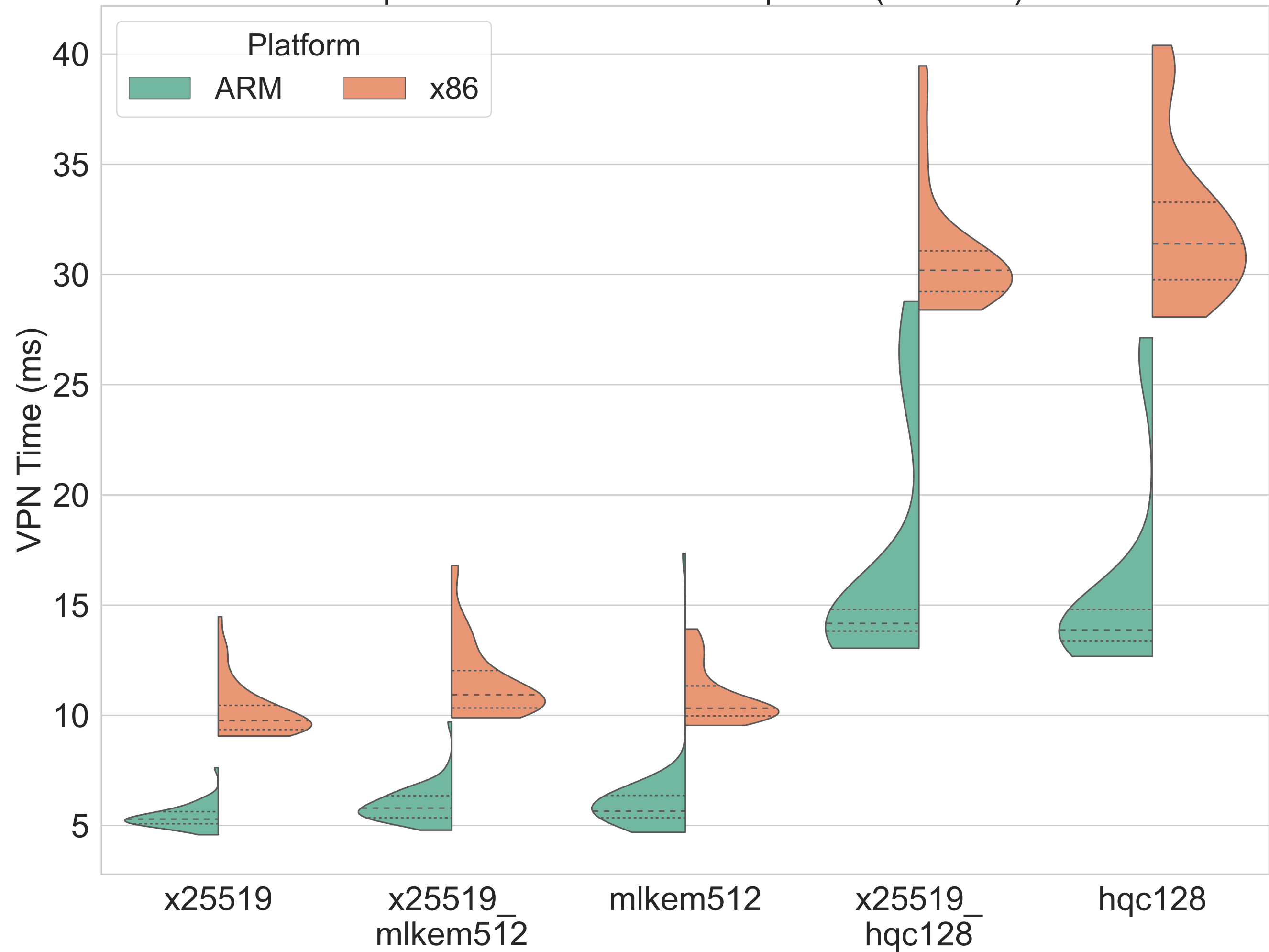
Impact of KEM on VPN Setup Time (ed25519)
