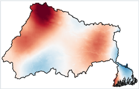
What we produce 9,538 cells, 0.1°
