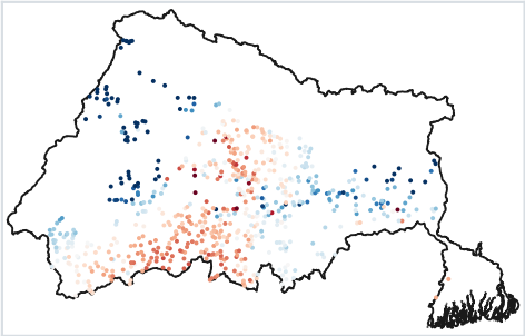
Checked against wells 656 wells
