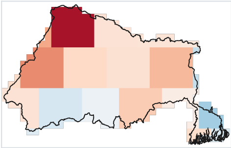
What GRACE sees 19 mascons, 3°
