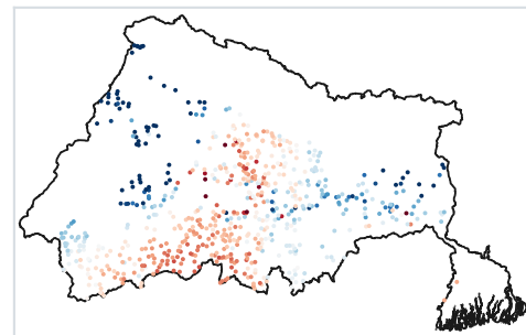
Checked 656 wells
