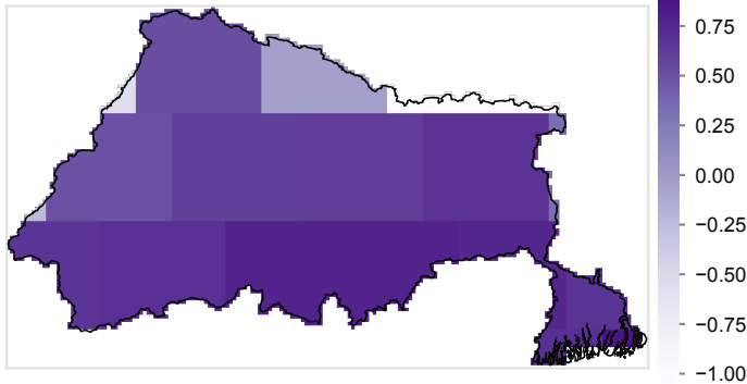
(c) NSE
