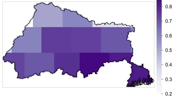
(b) R^2
