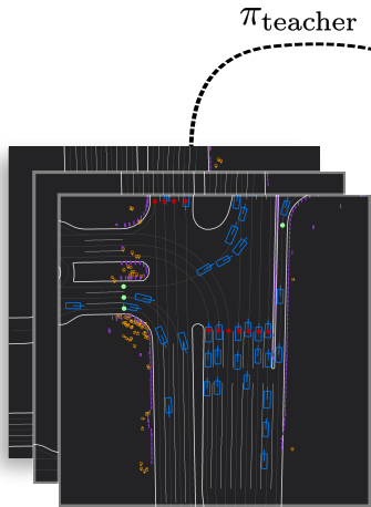
(a) Vectorized Self-Play RL
