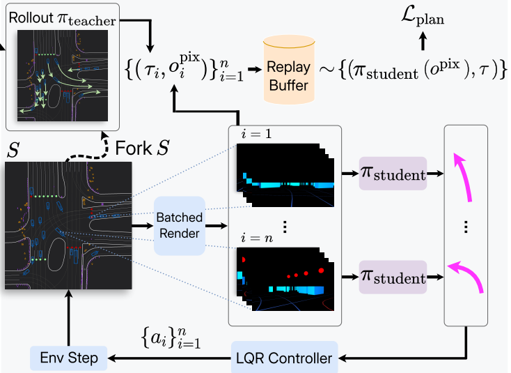
(b) Pixel-based Self-Play DAGger in Gigapixel
