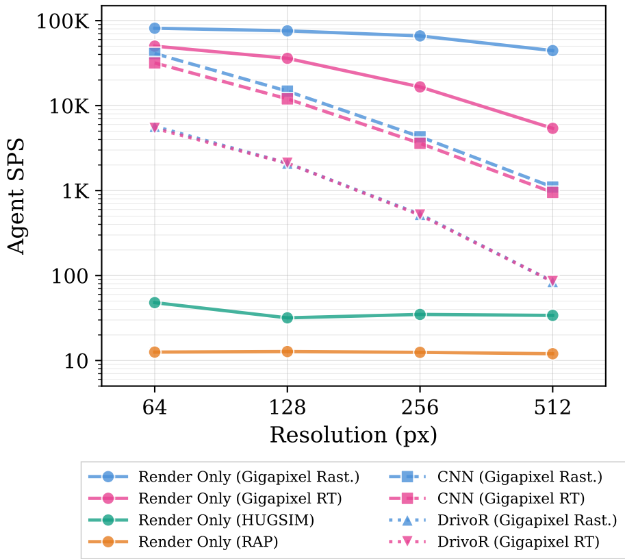
Agent SPS vs. Resolution
