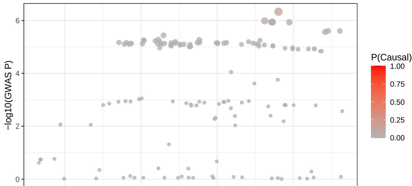
4_103732441 – edQTL Signal
