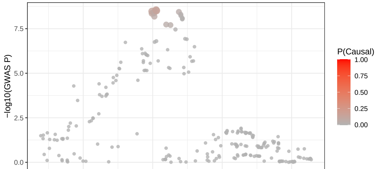
7_137067935 – edQTL Signal
