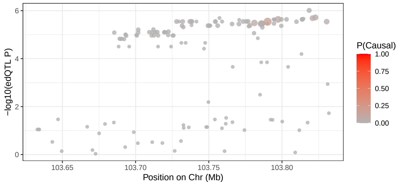
4_103732420 – edQTL Signal
