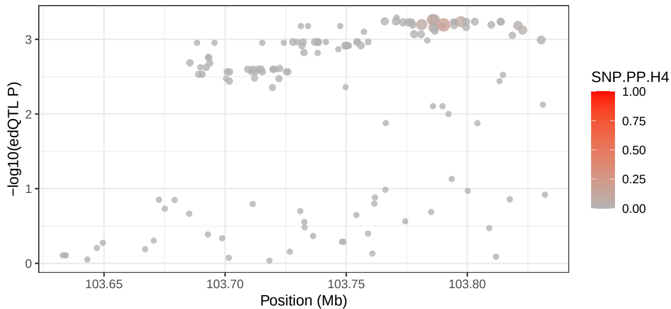
4_103732391 - edQTL
