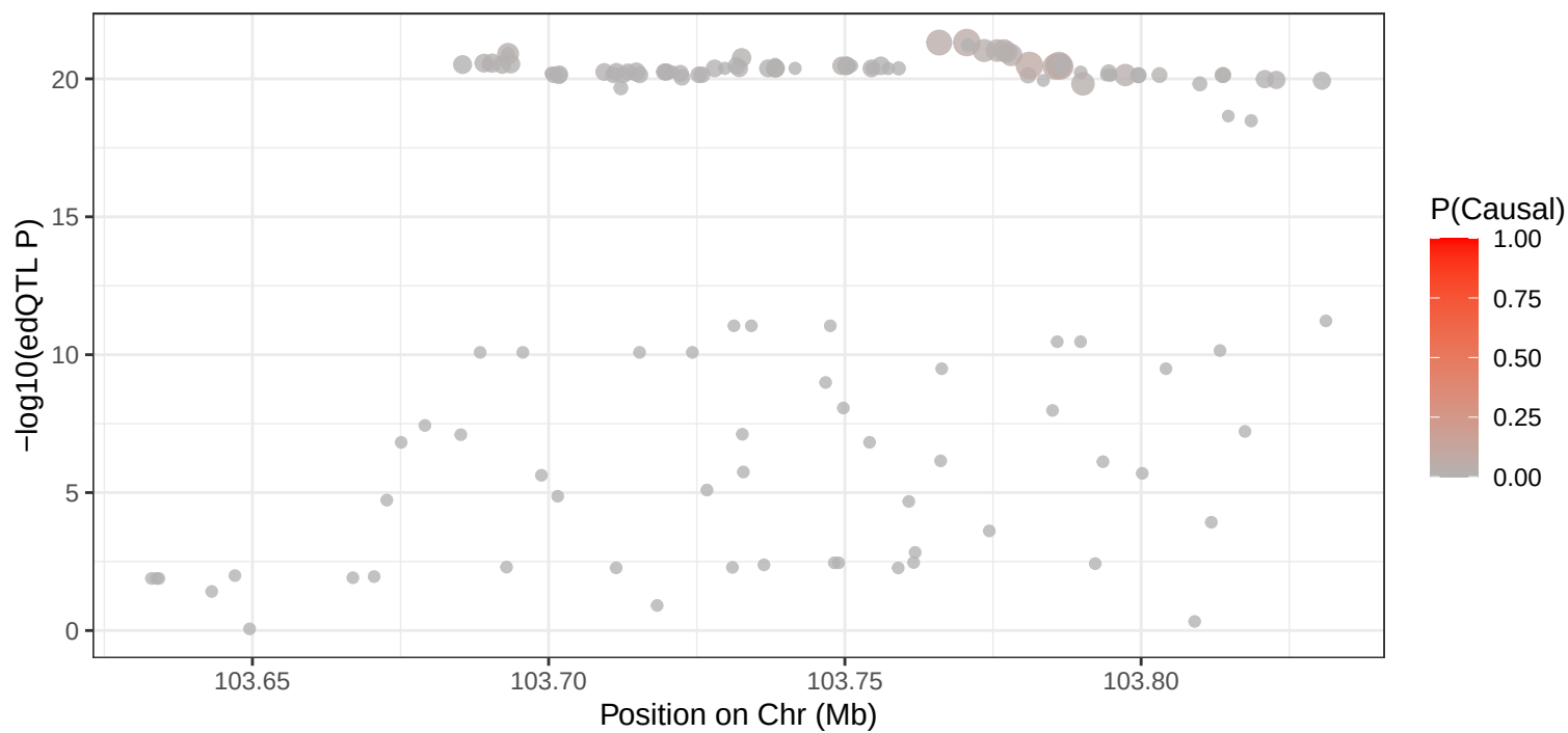
4_103731698 – edQTL Signal
