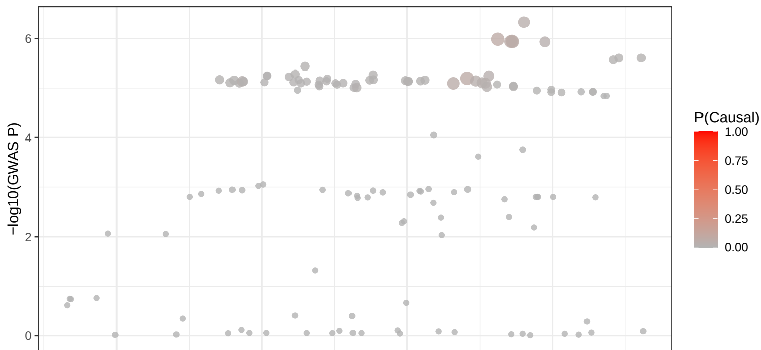
4_103731698 – edQTL Signal
