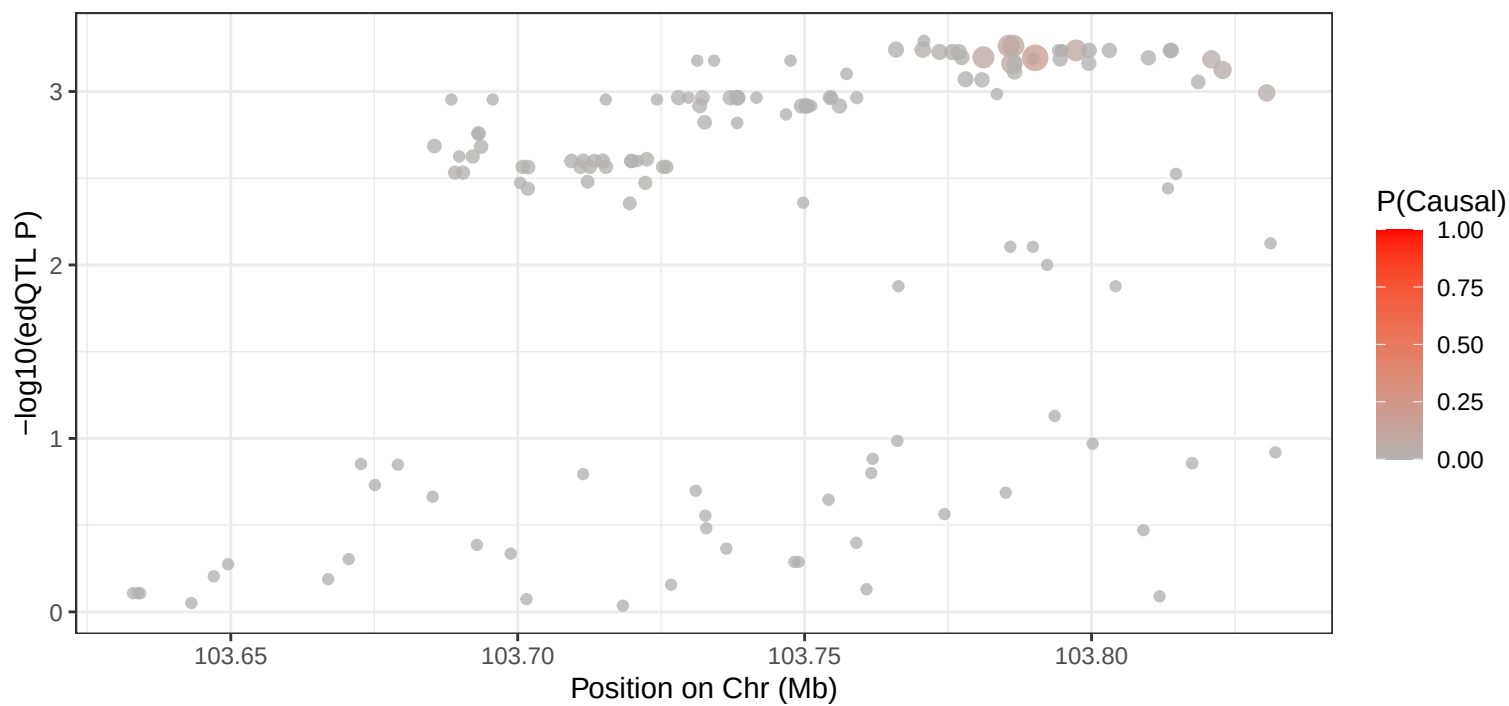
4_103732391 – edQTL Signal
