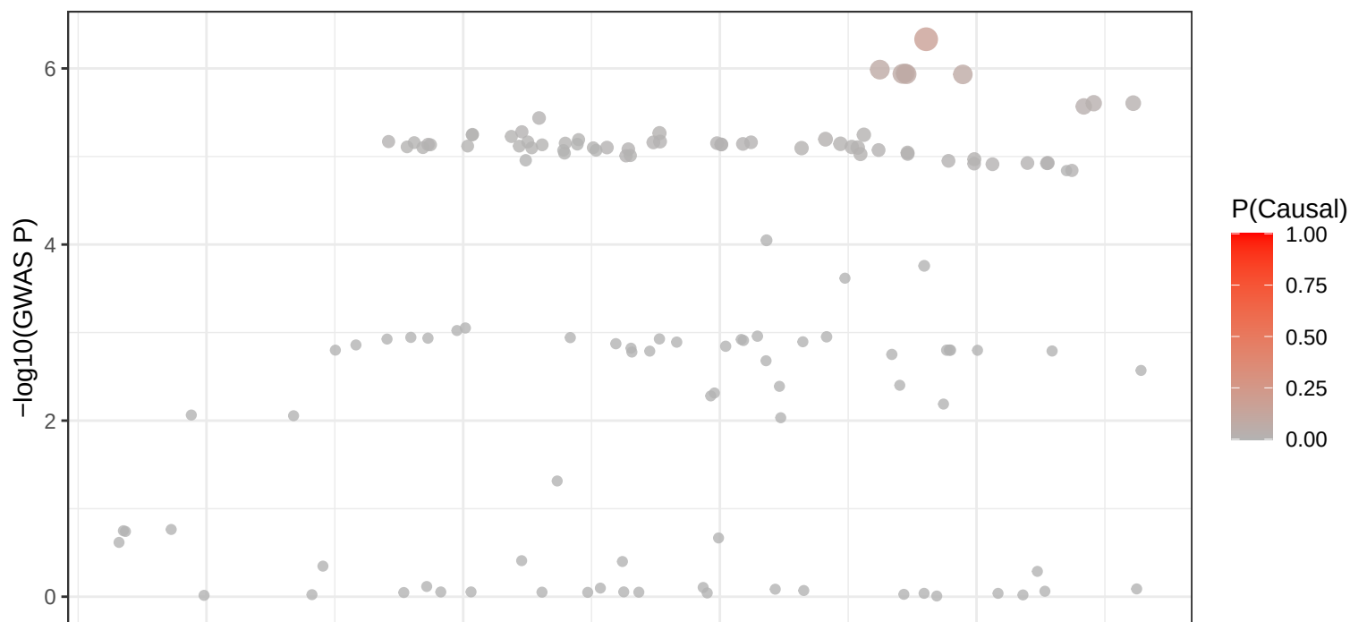
4_103732391 – edQTL Signal
