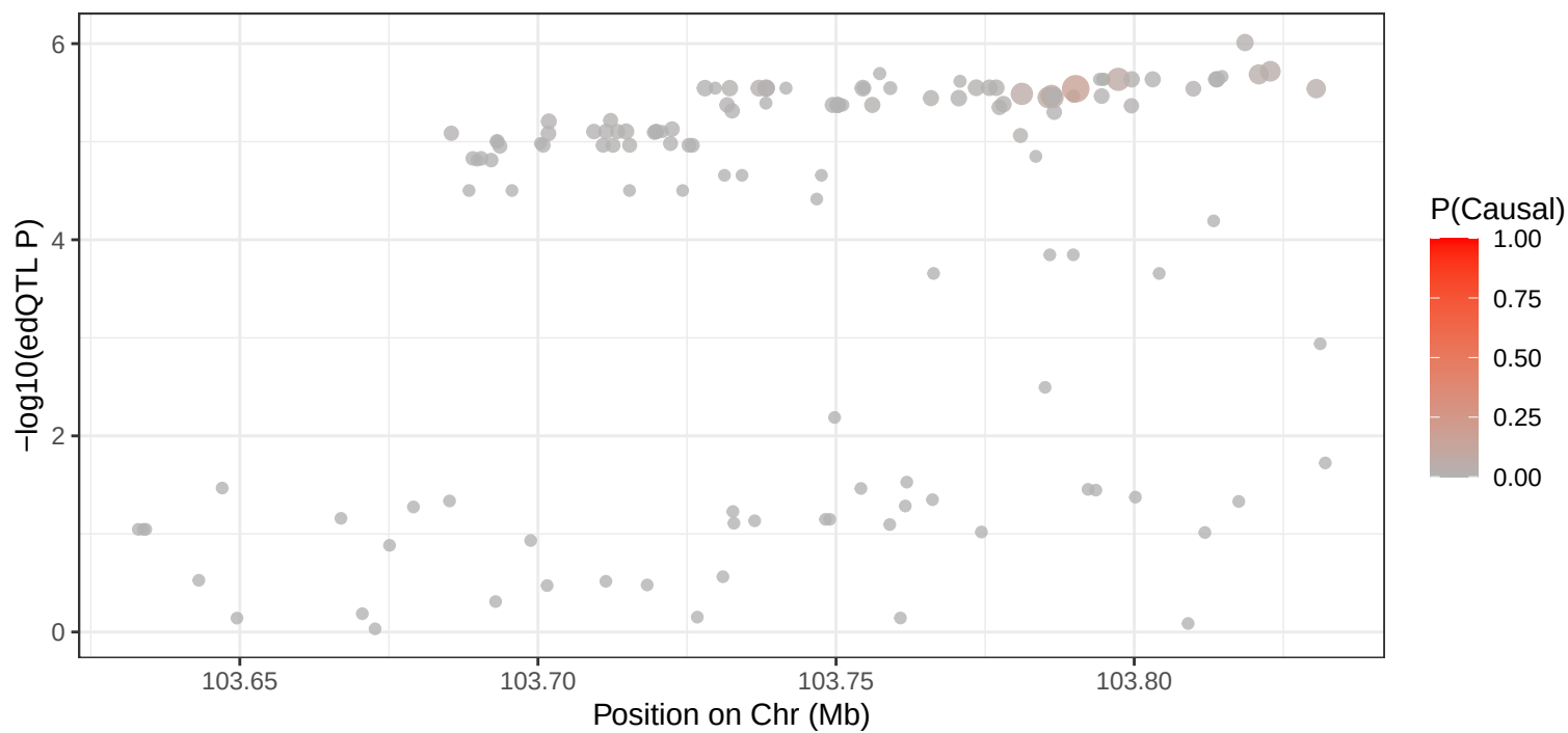
4_103732420 – edQTL Signal
