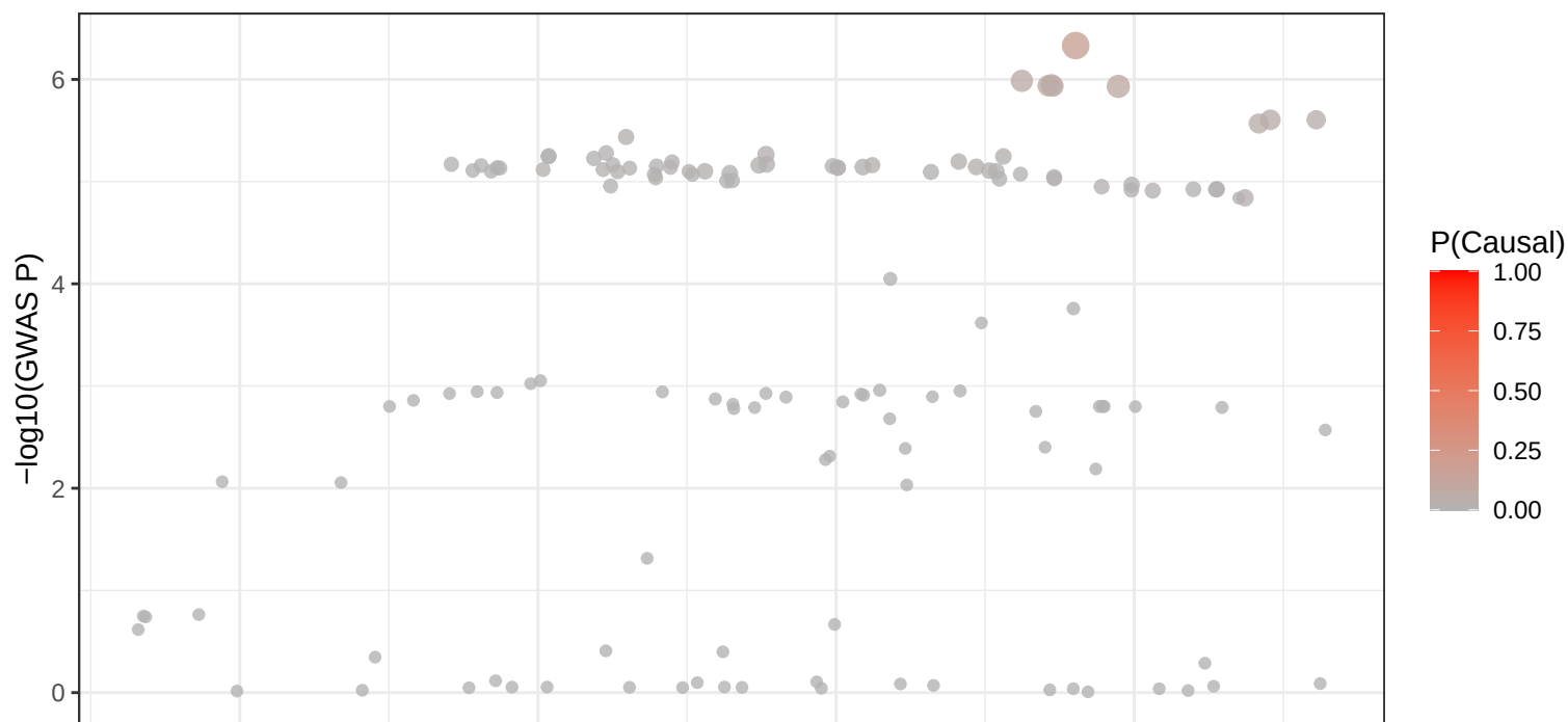
4_103732420 – GWAS Signal
