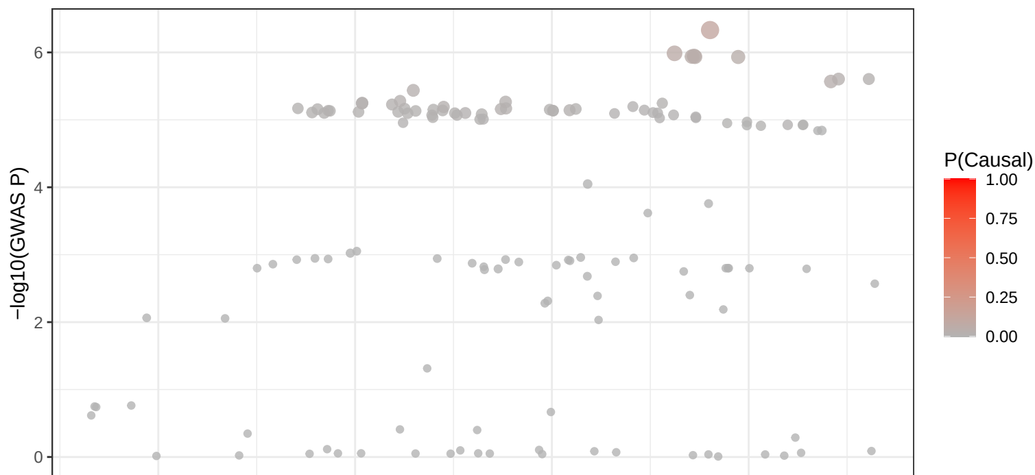
4_103732441 – edQTL Signal
