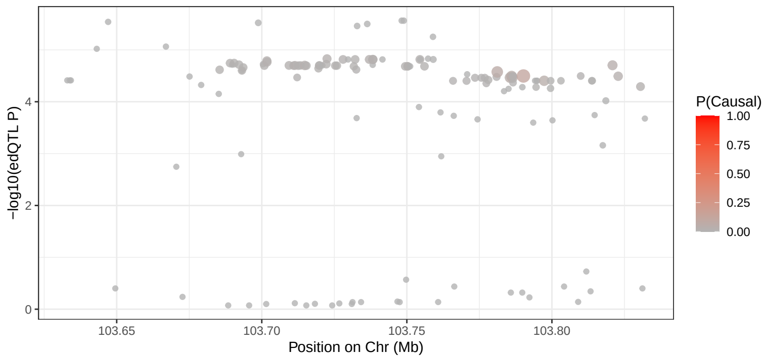
4_103732441 – edQTL Signal
