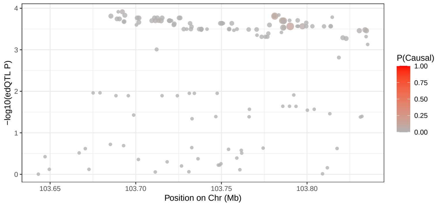
4_103735739 – edQTL Signal
