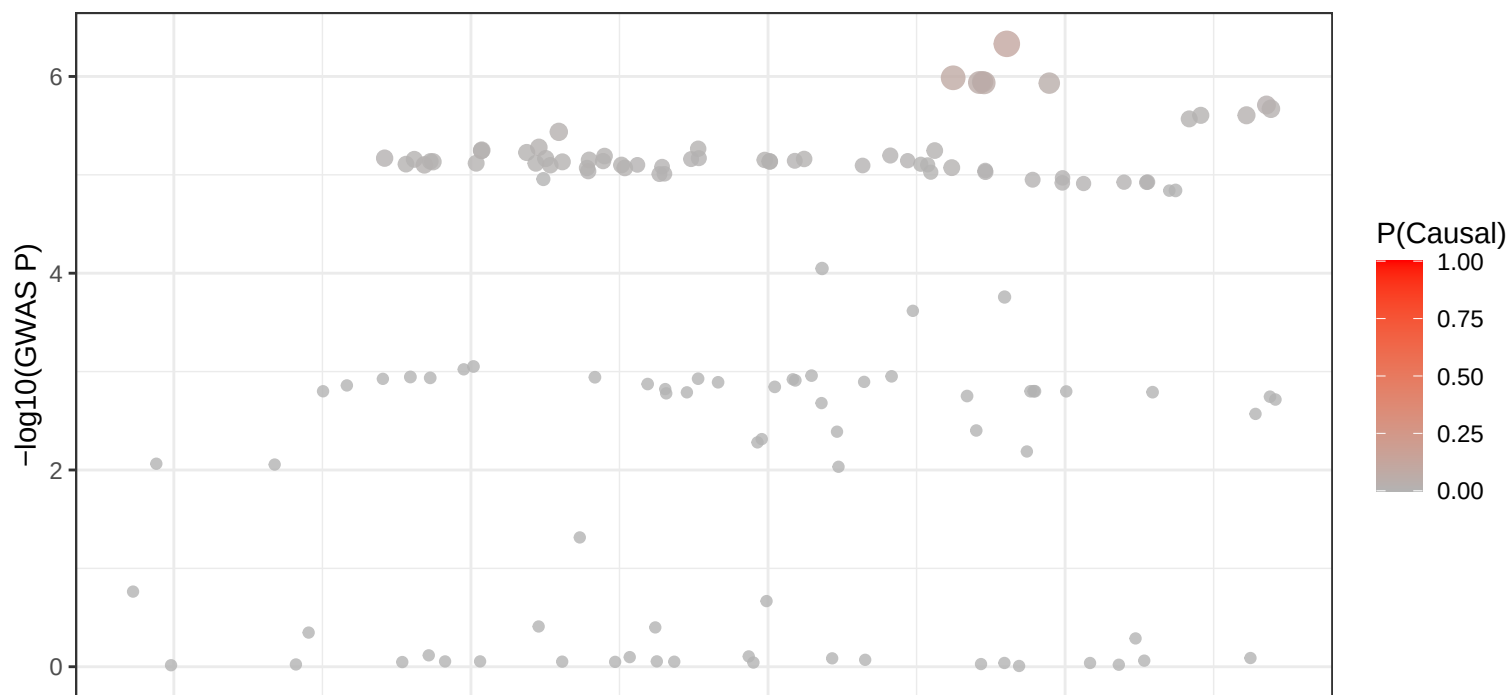
4_103735739 – edQTL Signal
