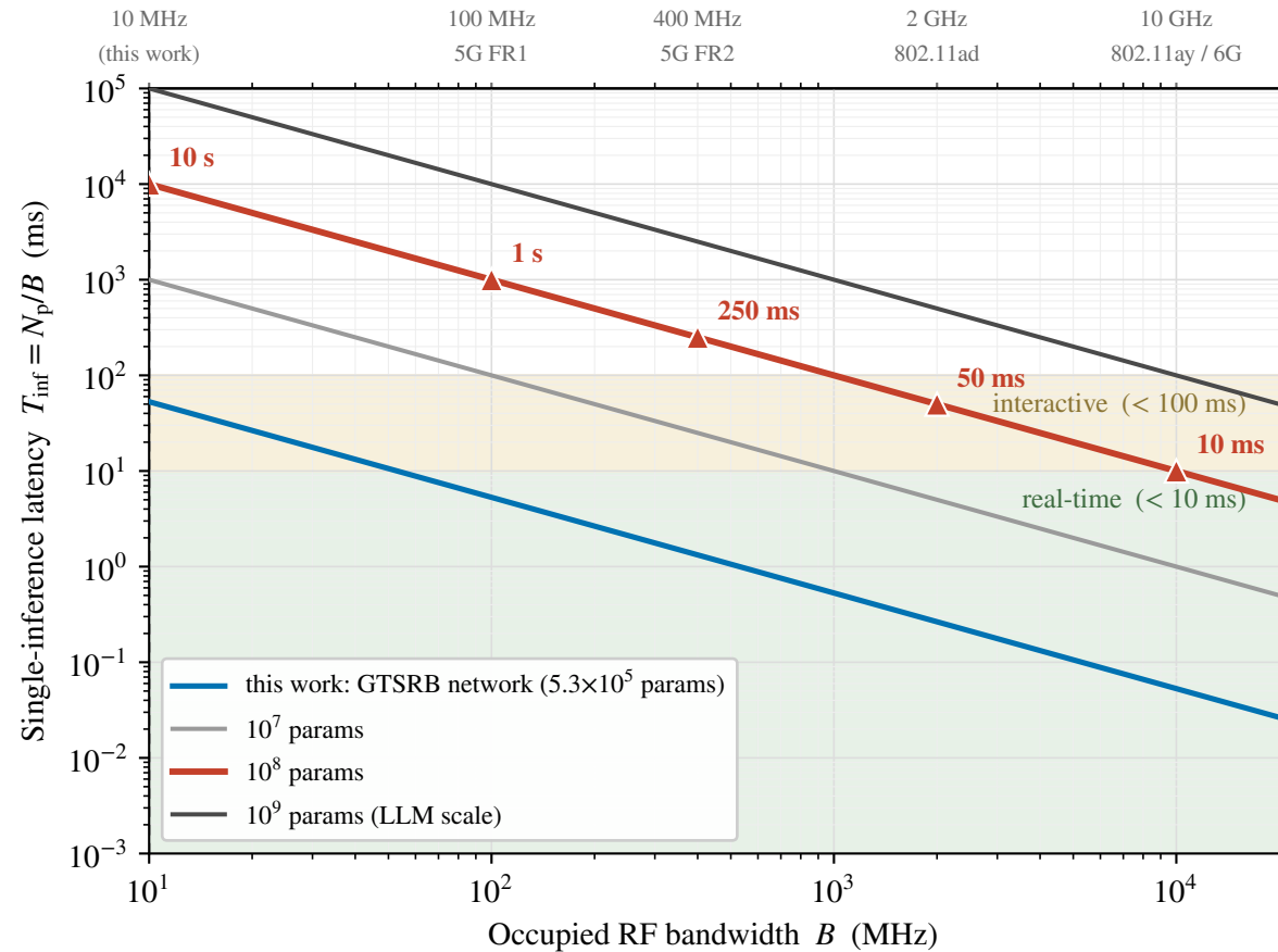
(a) Latency scales as N_p/B
