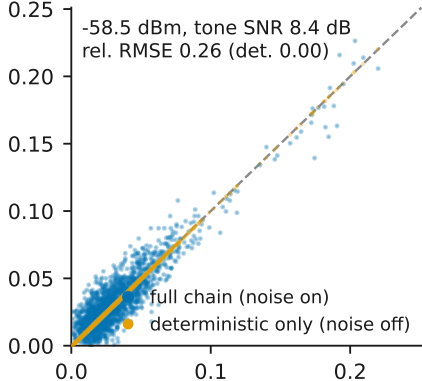
pass 3 (128 \rightarrow 43)
