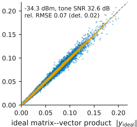
pass 2 (128 \rightarrow 128)
