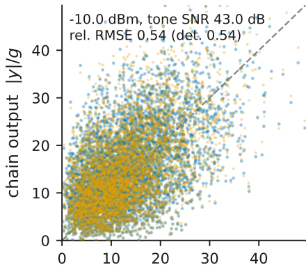
pass 1 (3072 \rightarrow 128)
