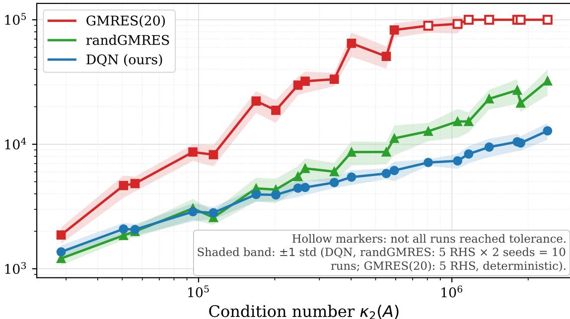
Total Arnoldi iterations vs. \kappa_2(A) on convection-diffusion matrices
