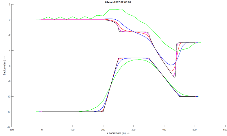
Figure 6.18: Top graphs present the water level. Lower graphs present the regularized bathymetry. Green: \Delta x = 20 [m], \Delta t = 4 [s]; Blue: \Delta x = 10 [m], \Delta t = 2 [s]; Red: \Delta x = 5 [m], \Delta t = 1 [s]; Cyan: \Delta x = 2.5 [m], \Delta t = 0.5 [s]; Black: \Delta x = 1.25 [m], \Delta t = 0.25 [s]
