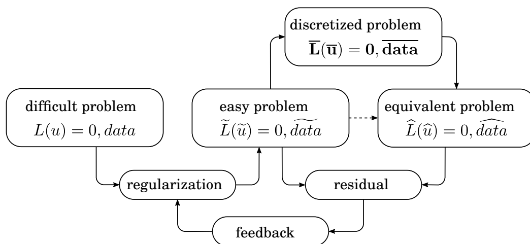
Figure 2.1: Graphical presentation of the error-minimizing two step method
