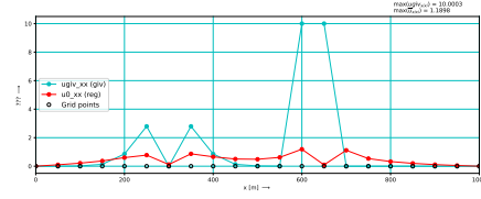
(b) Second derivatives, normalized grid size \Delta \xi = 1 .
