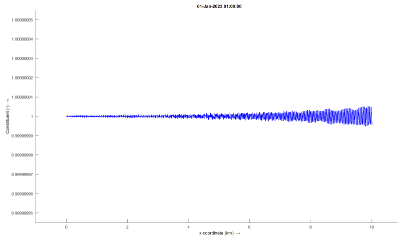
Figure 6.5: Constituent at t = 3600 [s]. Range of y -axis is from 1 \pm 5 \times 10^{-8} .
