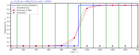
(b) Step defined with an of set of 0.3 \Delta x from cell centre.
