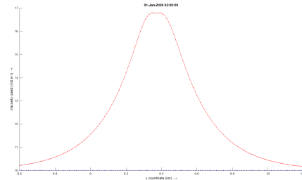
(b) Used artificial viscosity \Psi along channel at 2 [h]. The blue line, no artificial viscosity ( \nu + \Psi = 10 ) and the red line the used artificial viscosity.
