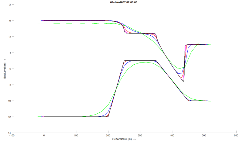
Figure 6.21: Top graphs present the water level. Lower graphs present the regularized bathymetry. Green: \Delta x = 20 [m], \Delta t = 4 [s]; Blue: \Delta x = 10 [m], \Delta t = 2 [s]; Red: \Delta x = 5 [m], \Delta t = 1 [s]; Cyan: \Delta x = 2.5 [m], \Delta t = 0.5 [s]; Black: \Delta x = 1.25 [m], \Delta t = 0.25 [s]
