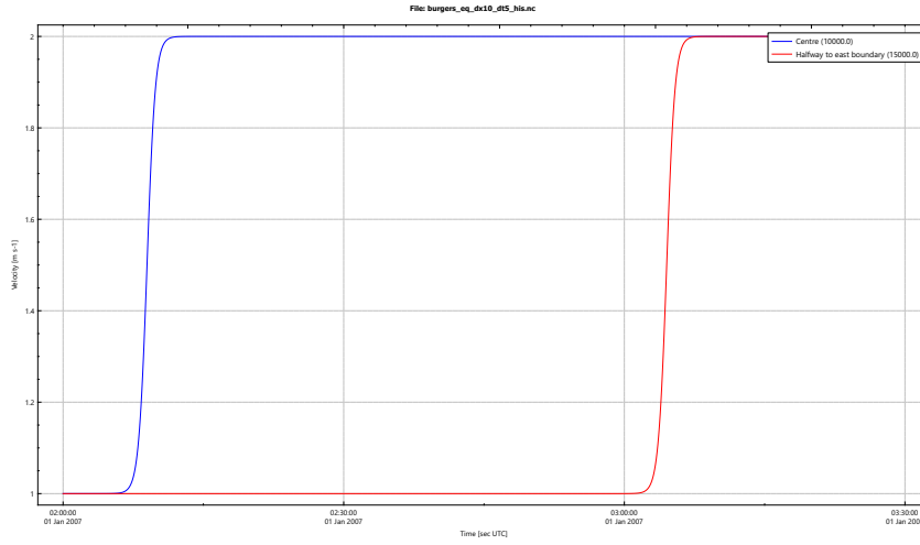
(a) Time histories of the velocity for the observation point at the x = 10\,000 [m] (blue line) and at x = 15\,000 [m] (red line).
